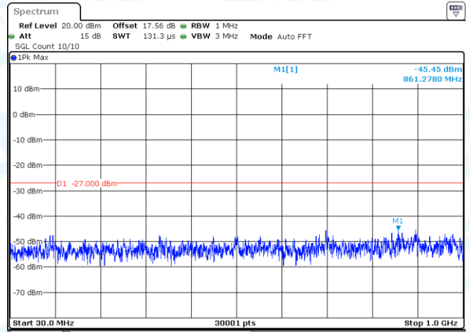
11AC20-CDD-Ant2-5260-30~1000-PASS
