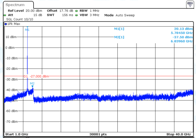
11AC20-CDD-Ant2-5785-1000~40000-PASS
