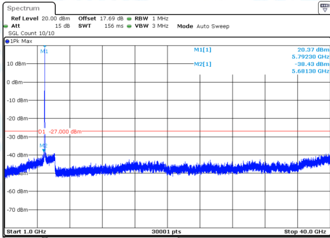
11AC20-CDD-Ant1-5785-1000~40000-PASS
