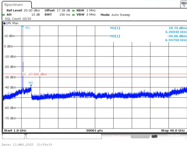
11AC20-CDD-Ant1-5200-1000~40000-PASS
