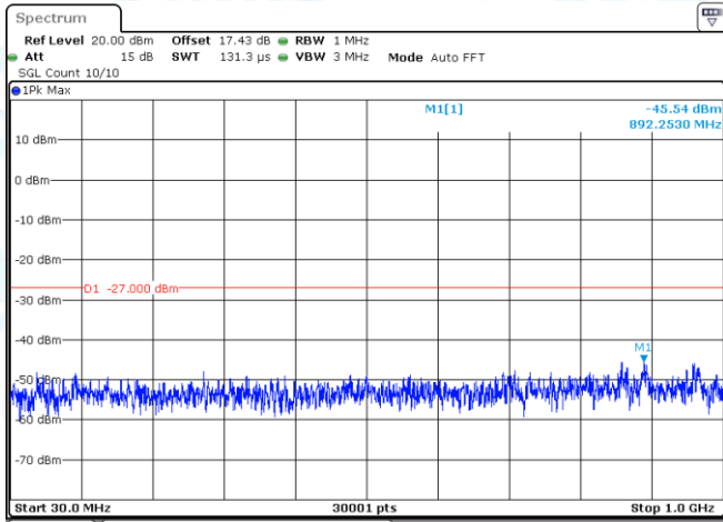
11N40-CDD-Ant1-5310-30~1000-PASS
