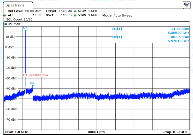
11N40-CDD-Ant2-5510-1000~40000-PASS
