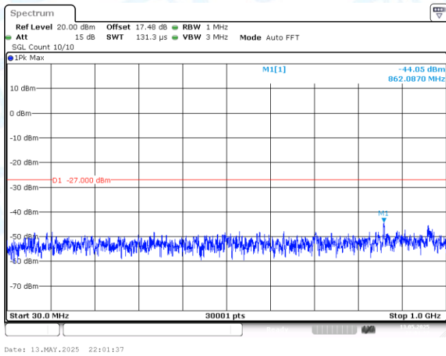
11AC20-CDD-Ant1-5240-30~1000-PASS
