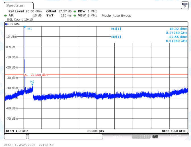
11AC20-CDD-Ant2-5240-1000~40000-PASS
