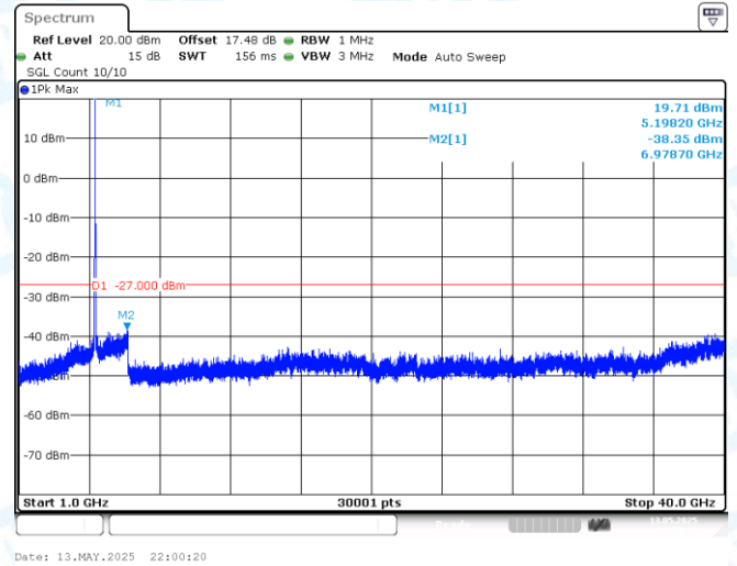
11AC20-CDD-Ant2-5200-1000~40000-PASS
