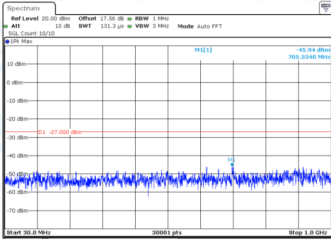
11AC20-CDD-Ant1-5500-30~1000-PASS
