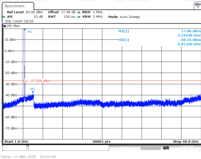
11AC20-CDD-Ant1-5240-1000~40000-PASS
