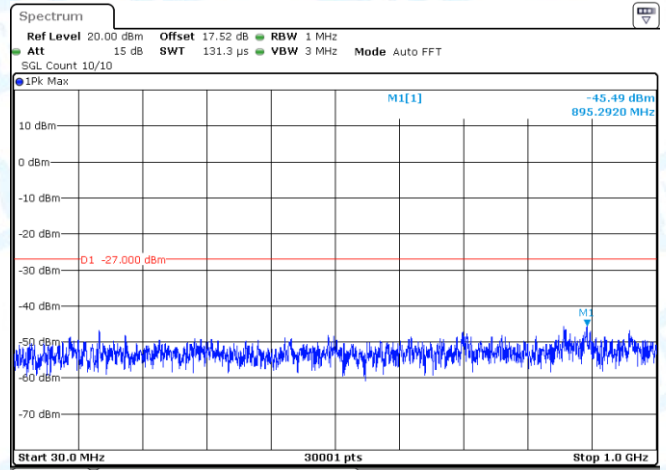
11N40-CDD-Ant2-5310-30~1000-PASS
