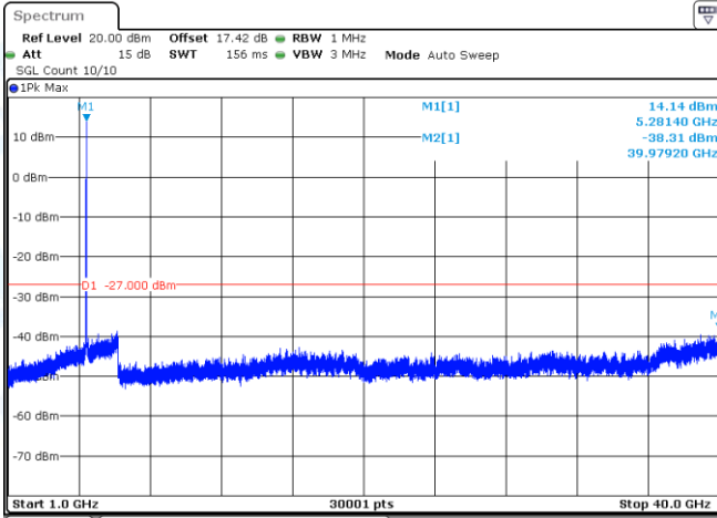
11N20-CDD-Ant1-5280-1000~40000-PASS
