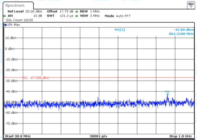
11N20-CDD-Ant2-5745-30~1000-PASS
