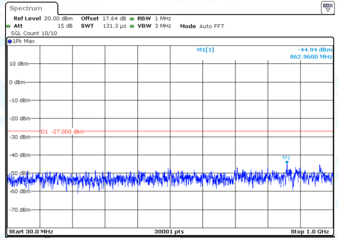
11N20-CDD-Ant2-5500-30~1000-PASS
