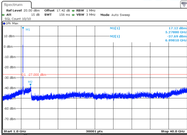
11A-Ant1-5280-1000~40000-PASS
