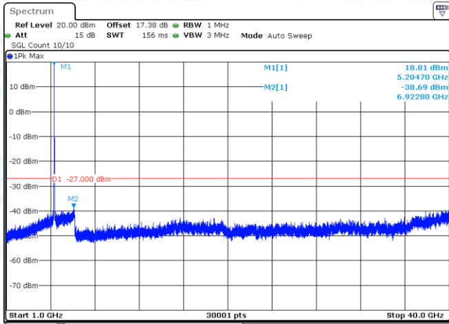
11N20-CDD-Ant1-5200-1000~40000-PASS
