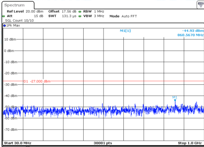
11N20-CDD-Ant1-5500-30~1000-PASS
