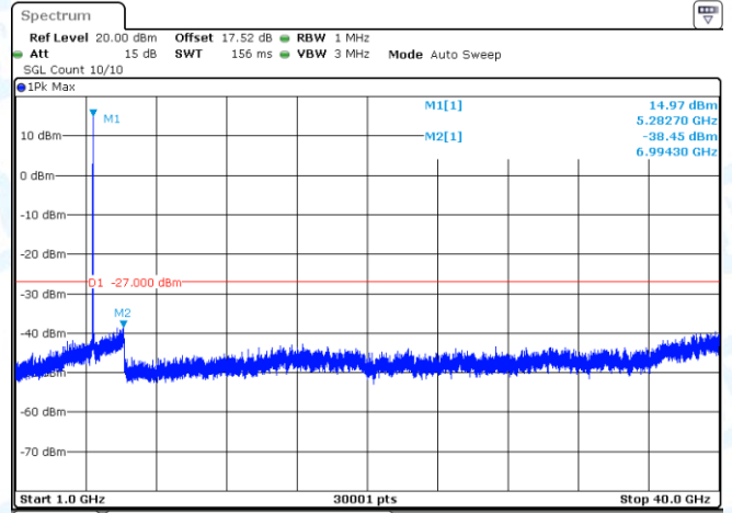
11N20-CDD-Ant2-5280-1000~40000-PASS
