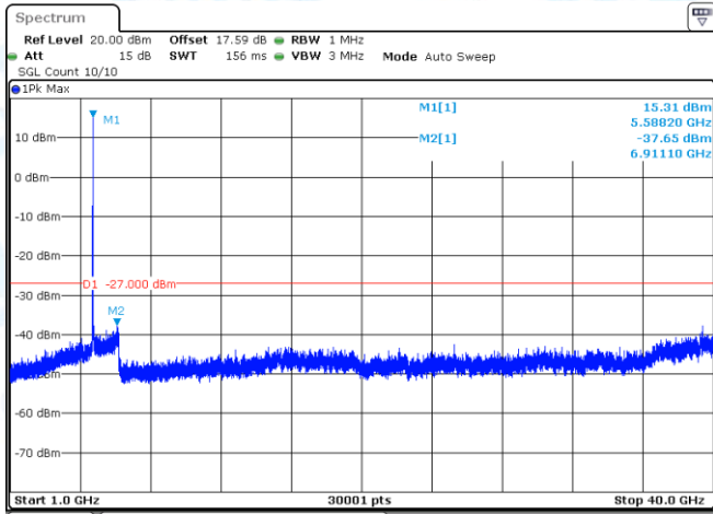
11N20-CDD-Ant1-5580-1000~40000-PASS
