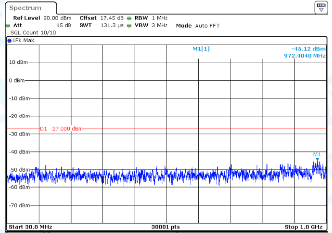
11N20-CDD-Ant1-5180-30~1000-PASS
