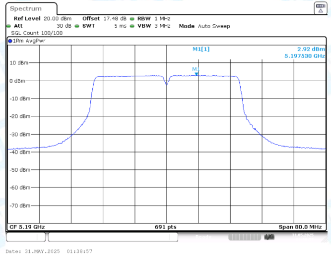
11N40-CDD-Ant2-5190-PASS
