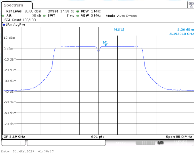
11N40-CDD-Ant1-5190-PASS
