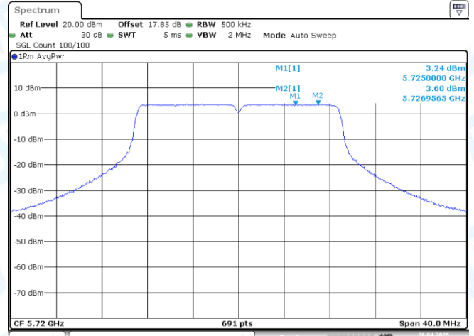
11AC20-CDD-Ant2-5720_UNII-3-PASS
