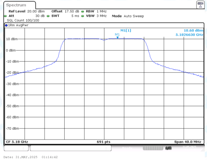
11A-Ant2-5180-PASS
