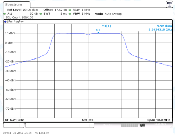
11A-Ant2-5240-PASS
