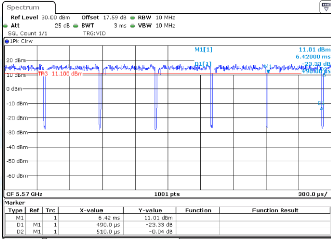
NTNV-11AX160-CDD-Ant1-5570
