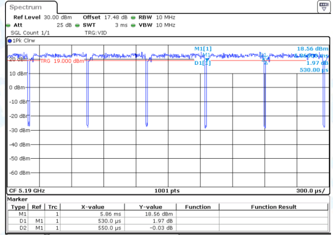
NTNV-11AX40-CDD-Ant2-5190
