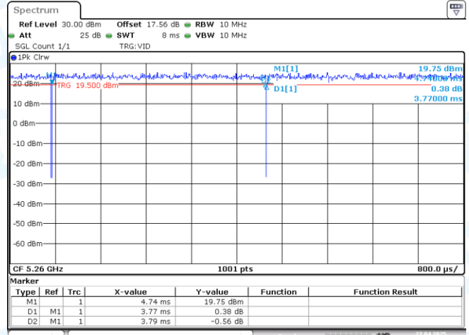
NTNV-11AX20-CDD-Ant2-5260
