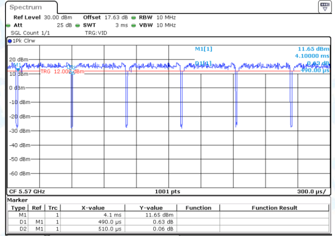
NTNV-11AX160-CDD-Ant2-5570
