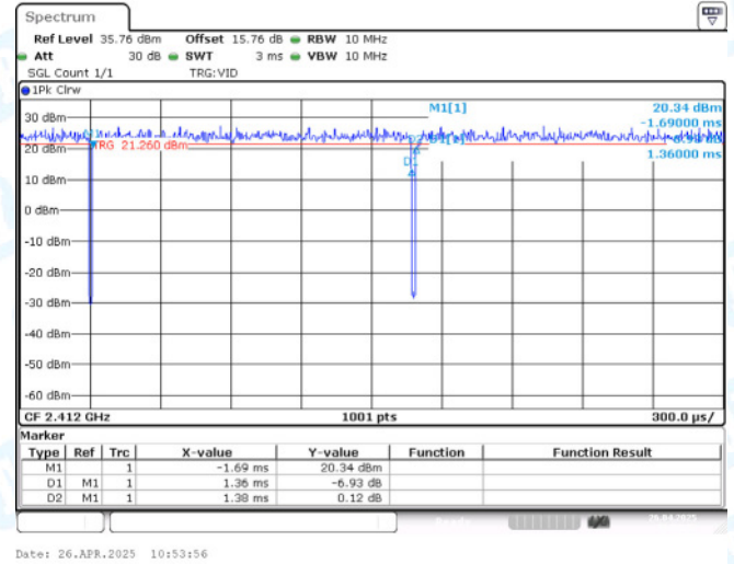
NTNV-11G-Ant2-2412
