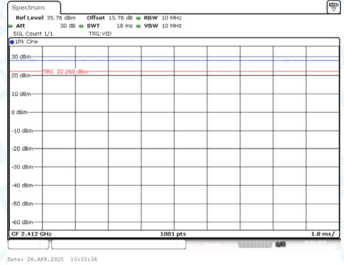
NTNV-11B-Ant2-2412
