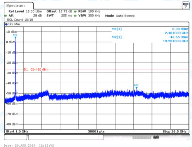
11AX20-CDD-Ant2-2462-1000~26500-PASS
