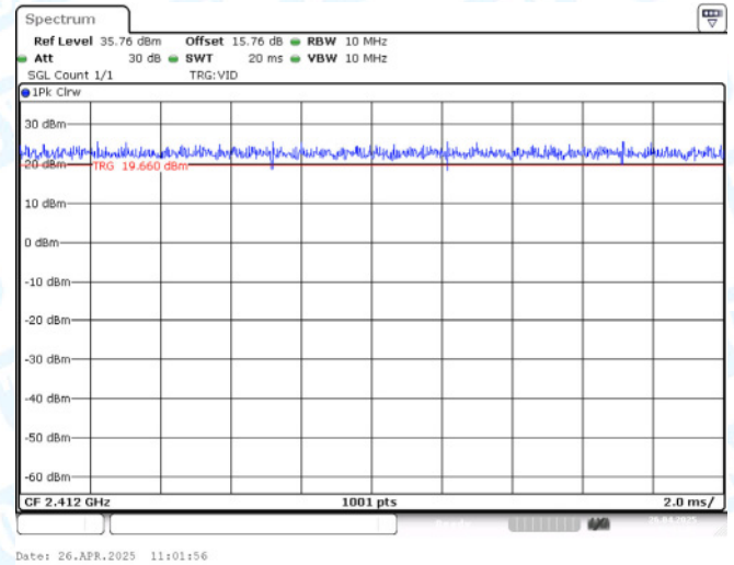
NTNV-11N20-CDD-Ant2-2412
