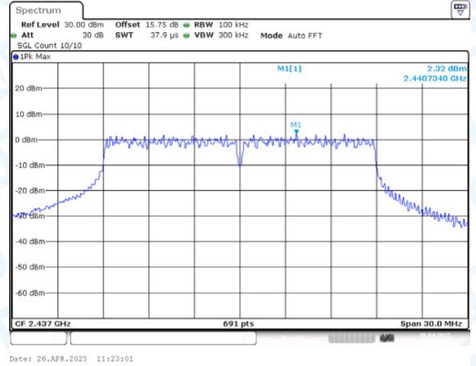
11N20-CDD-Ant2-2437-0~Reference-PASS
