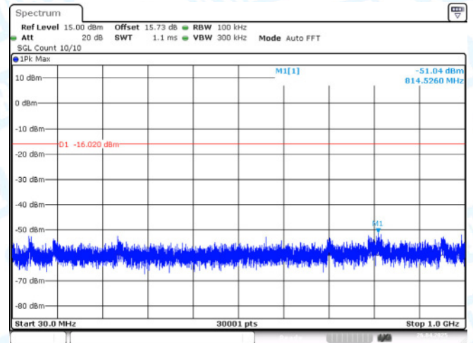
11B-Ant2-2462-0~Reference-PASS
