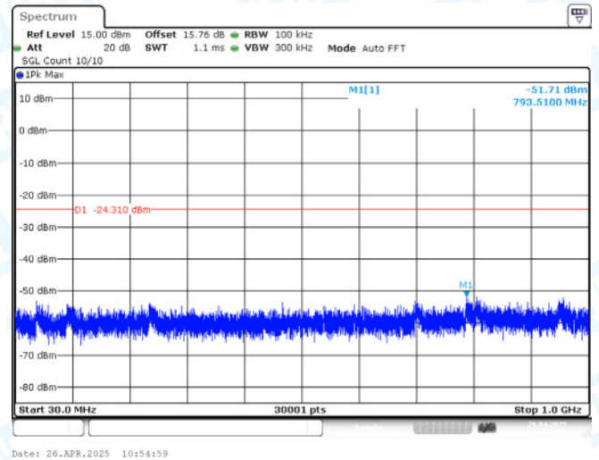
11G-Ant2-2412-30~1000-PASS
