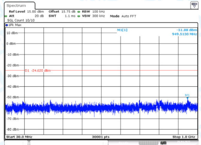
11AX20-CDD-Ant2-2437-0~Reference-PASS
