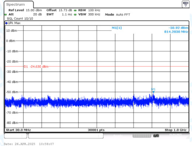
11G-Ant2-2462-30~1000-PASS
