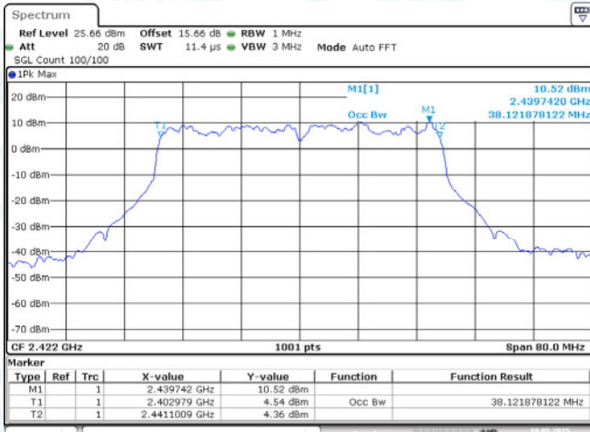
11AX40-CDD-Ant1-2422
