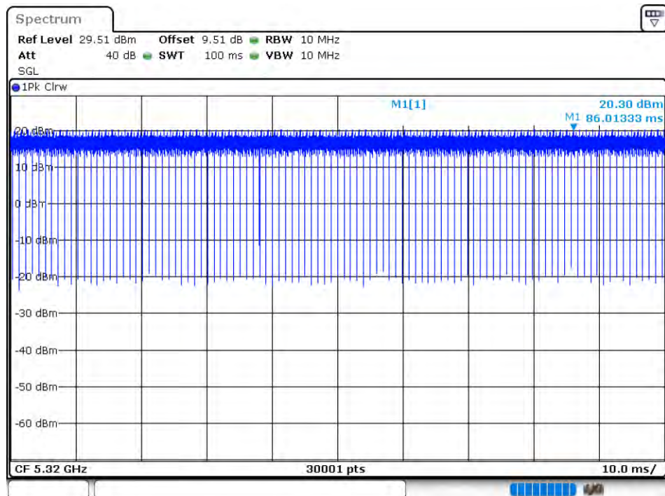
Duty Cycle NVNT 802.11ax20 5320MHz Ant 1
