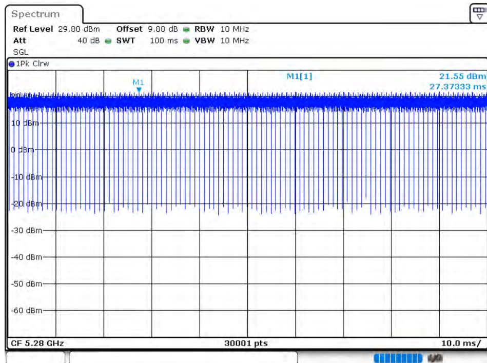
Duty Cycle NVNT 802.11ax20 5280MHz Ant 2
