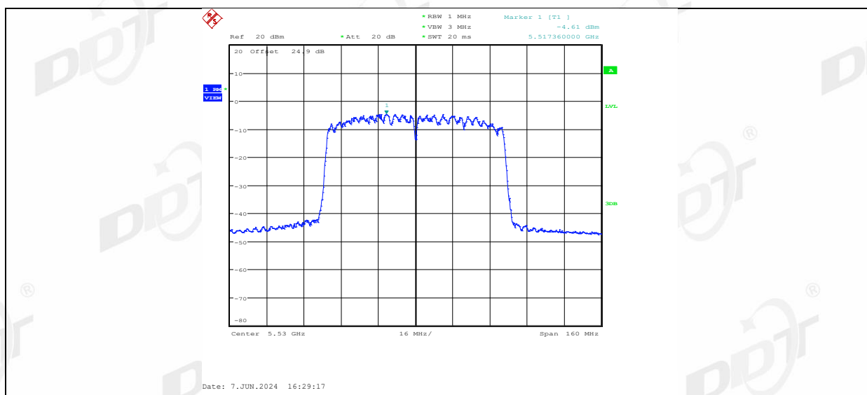
11AC80MIMO Ant2 5530
