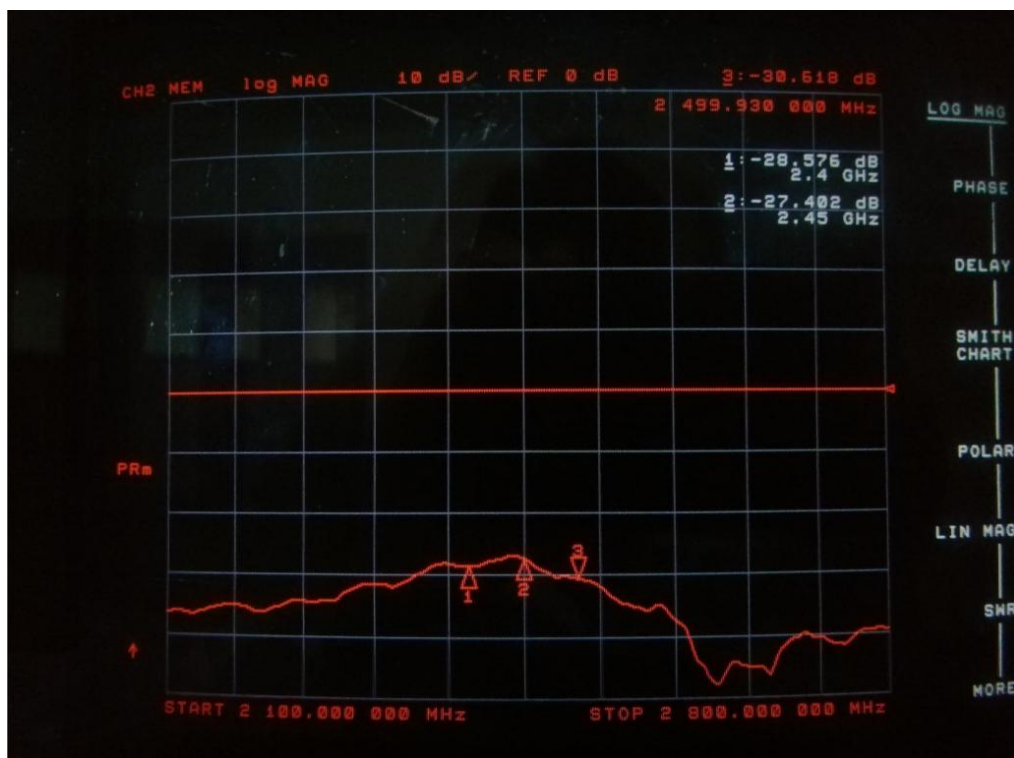
Isolation between WIFI-A and WIFI-B at 2.4G
