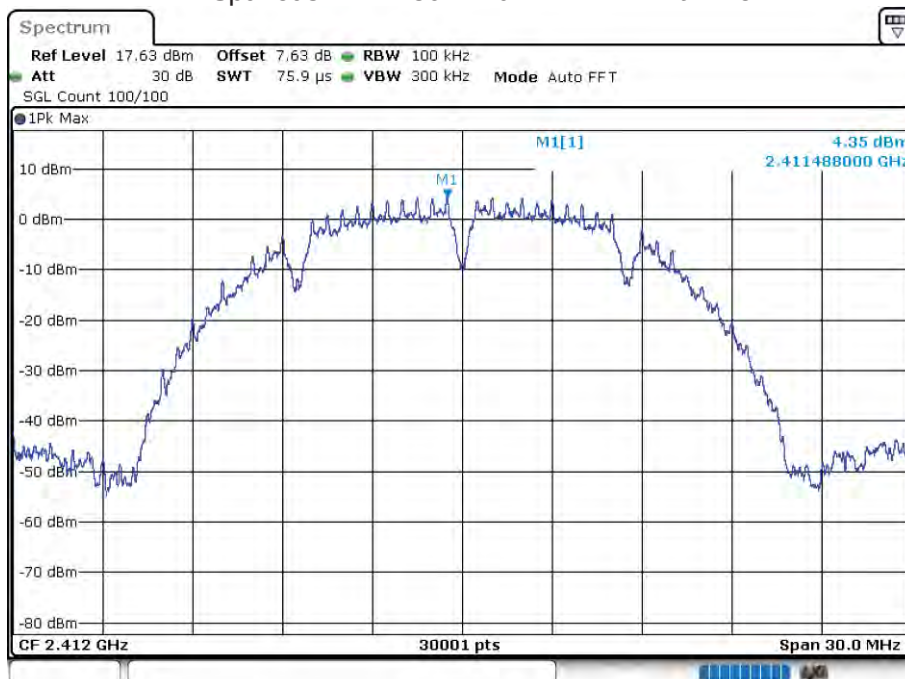
Tx. Spurious NVHT 802.11b 2412MHz Ant 1 Ref
