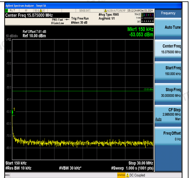
Band4-1312-0.15~30MHz-PASS
