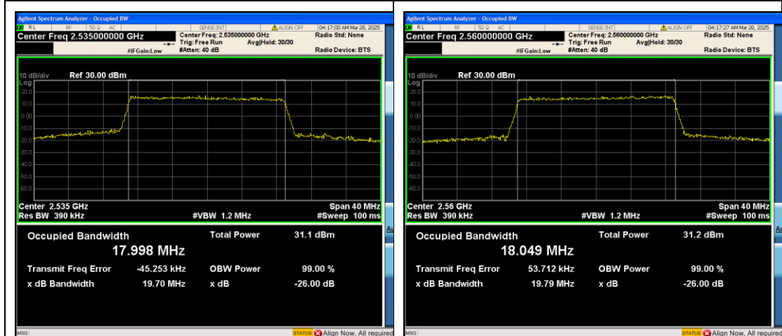
Band7-20MHz-16QAM-21100-100RB#0-PASS
