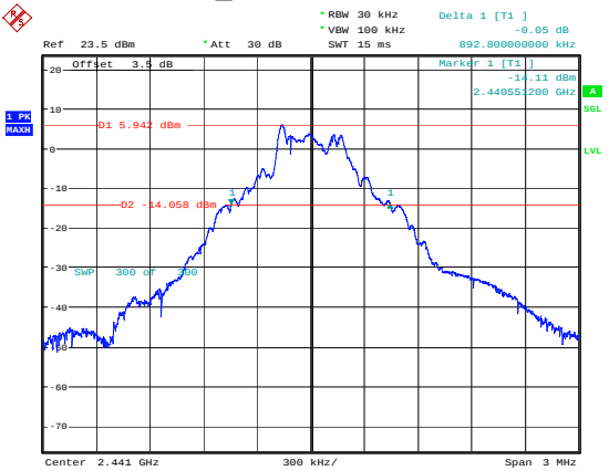
GFSK_Middle 0.893MHz
