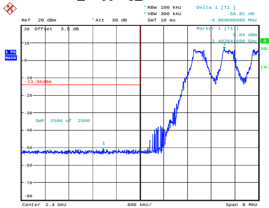
GFSK_Hopping_Lower 56.82dB
