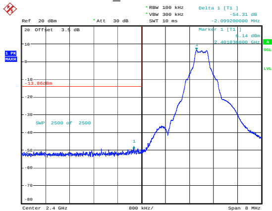
GFSK_Low 54.31dB
