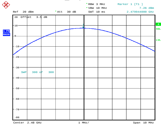
GFSK_High 7.26dBm
