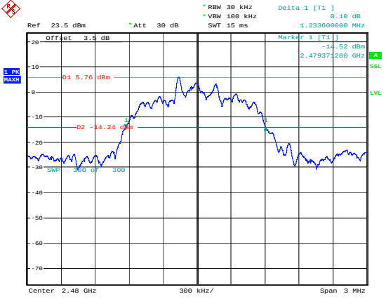
\pi/4 -DQPSK_High 1.234MHz
