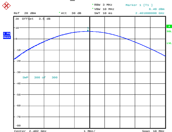
GFSK_Low 6.49dBm
