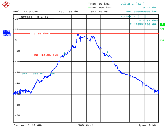
GFSK_High 0.893MHz
