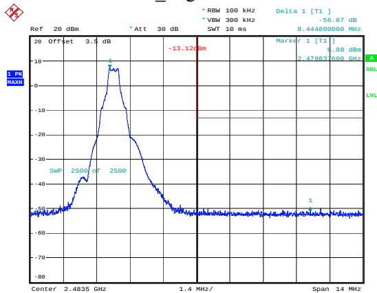
GFSK_High 56.67dB
