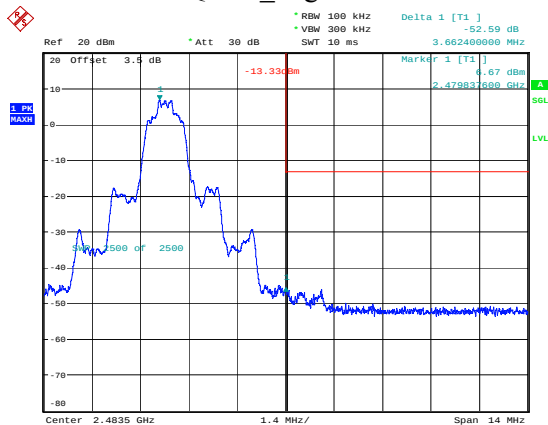
\pi/4 -DQPSK_High 52.59dB
