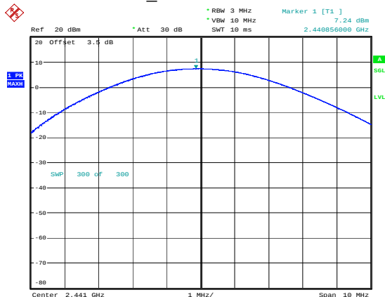
GFSK_Middle 7.24dBm
