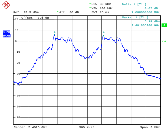
GFSK_Low 1.001MHz
