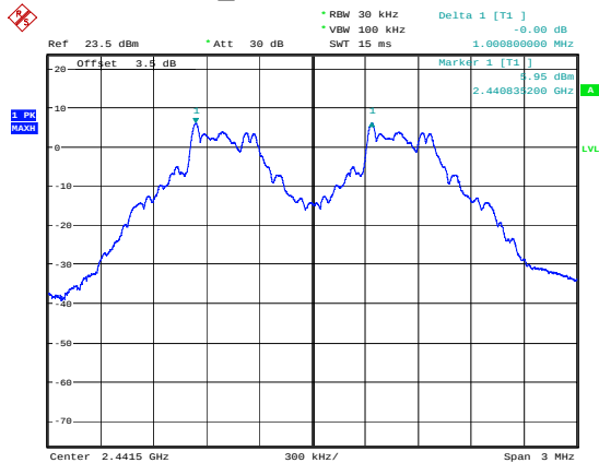
GFSK_Middle 1.001MHz
