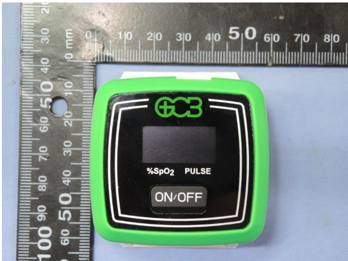
External View
