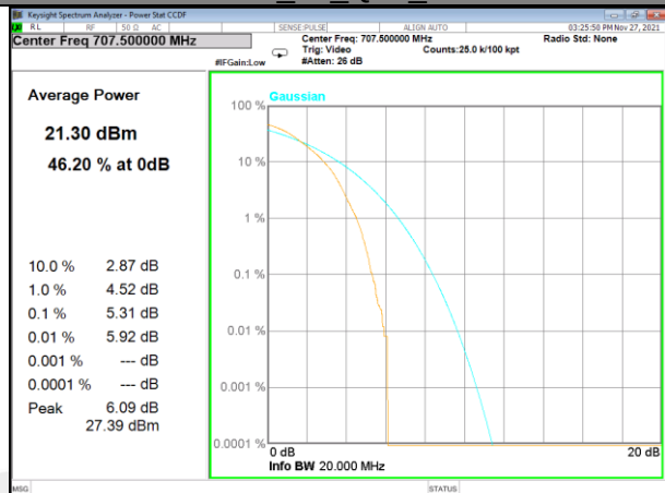
Band 12_50_QPSK_High
