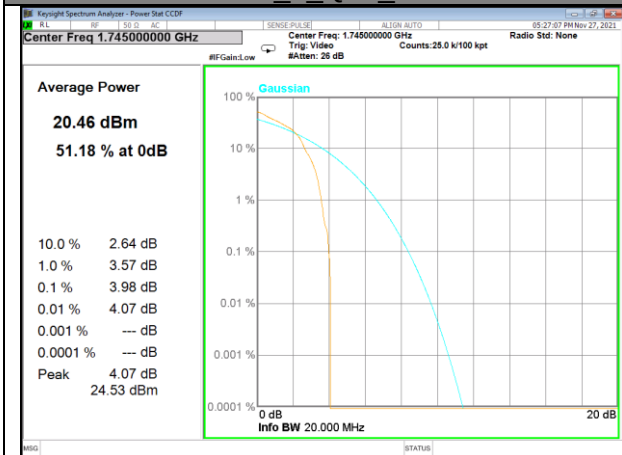
Band 66_1_QPSK_High
