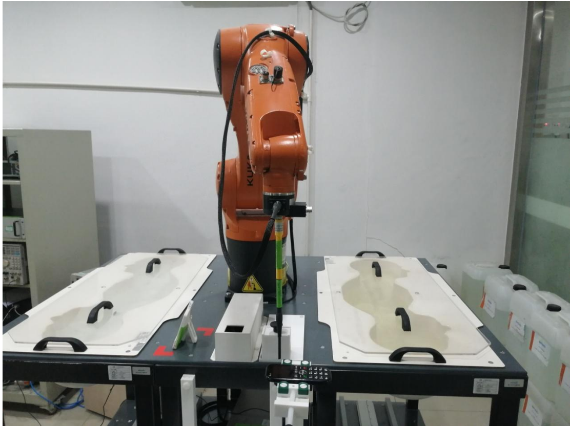
2AW56-EZ4G _HAC-Emissions Setup photo
