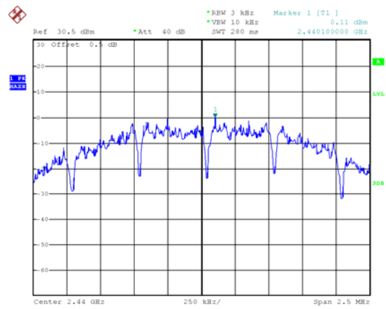
Mode: TX O-QPSK channel 7
