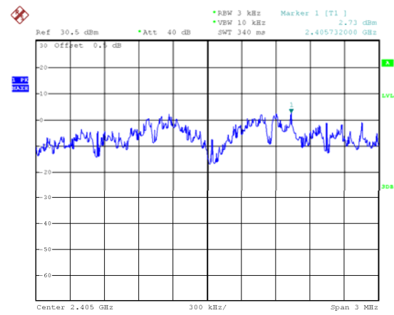
Mode: TX O-QPSK channel 0
