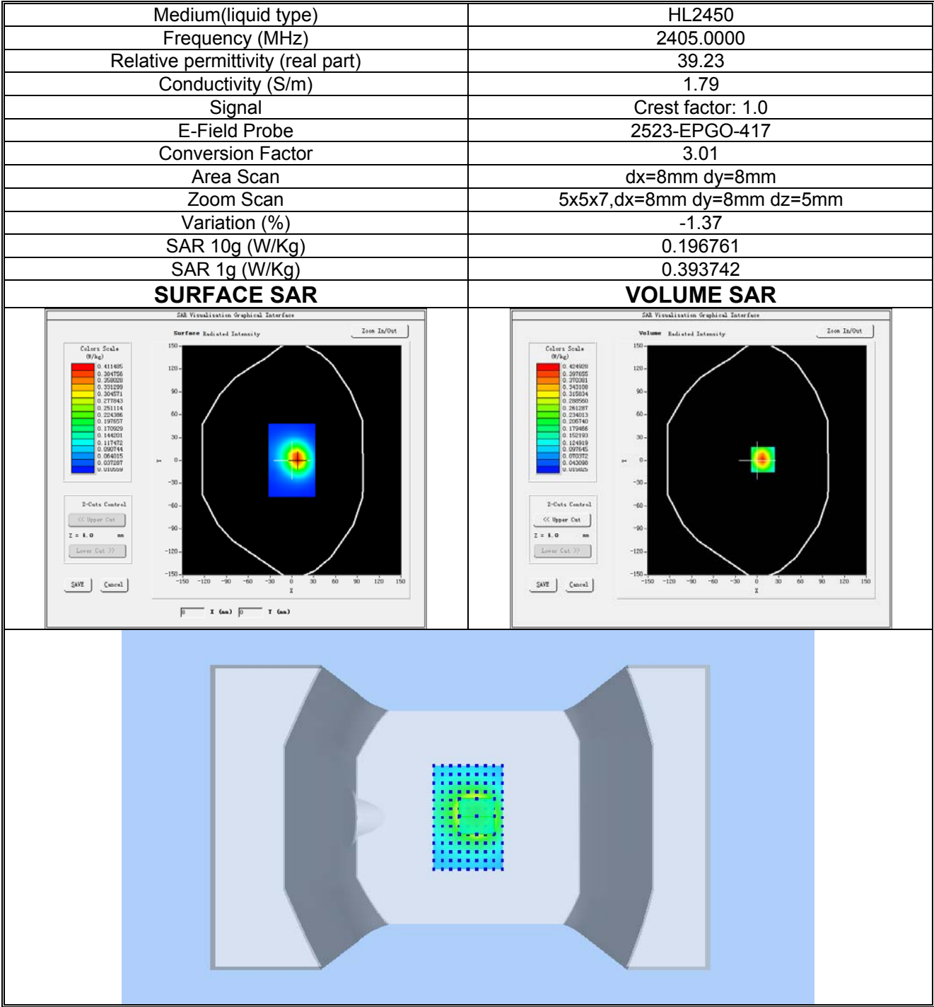
Plot 2: 2.4G SRD ANT 2, Low channel (Body SAR, Top Edge) Product Description: Spirit WAVE Test Date: 2024-09-29
