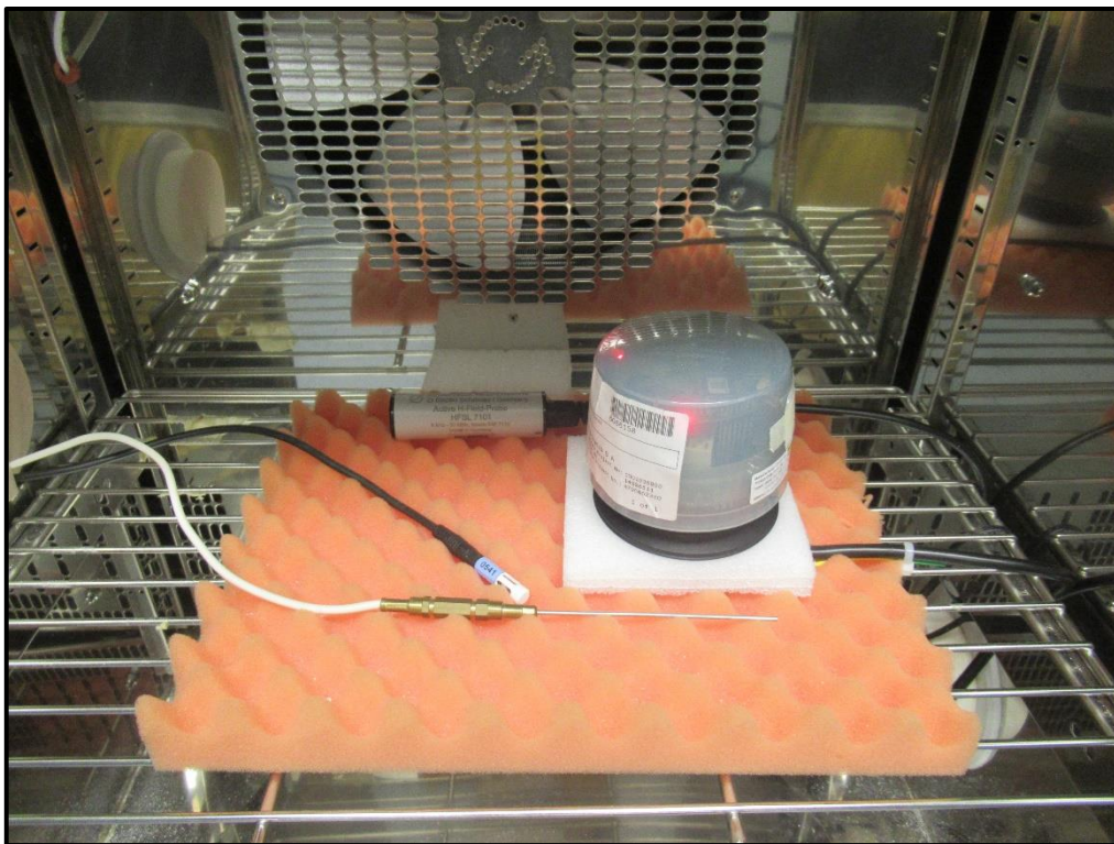
Photo 6 Bench test set up for (20 dB Bandwidth and Frequency Stability) (@ Ambient + Extreme Temperature, as required)
