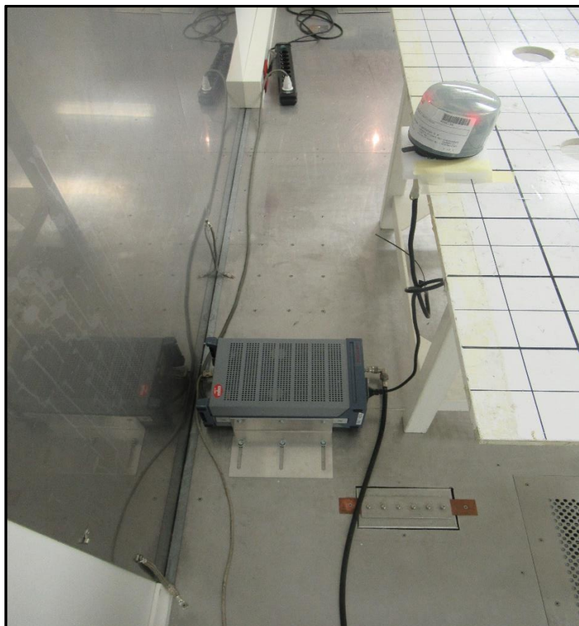
Photo 8 AC conducted emission
