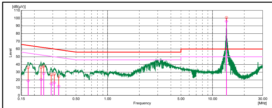
Plot: Neutral / 120 VAC 60 Hz
