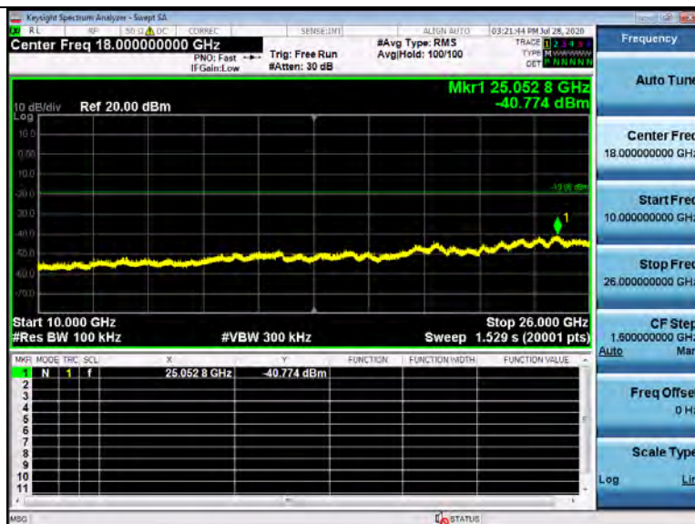
10GHz-26GHz
