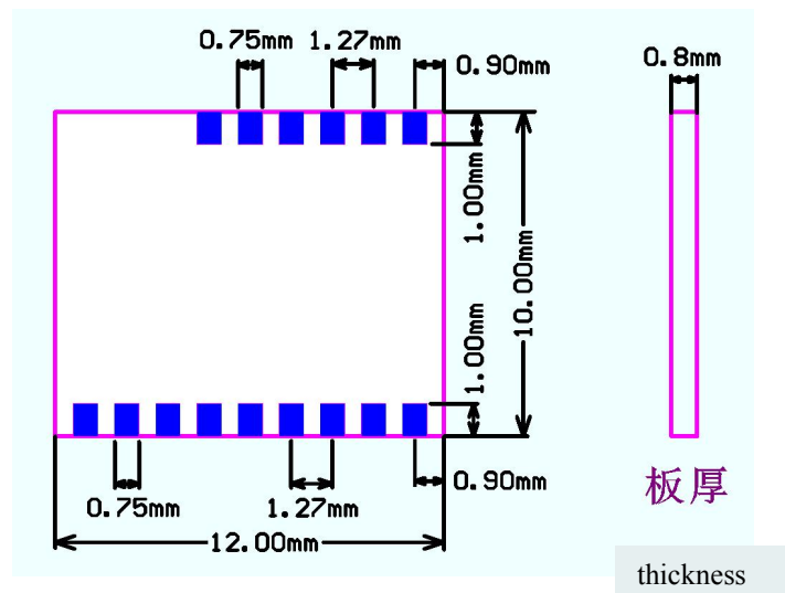
Fig 3.1 Package size chart (The overall maximum thickness of the module is 2.6mm)
