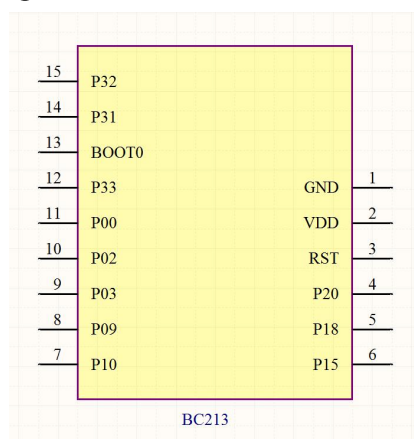
Fig 4.1 Pin Diagram
