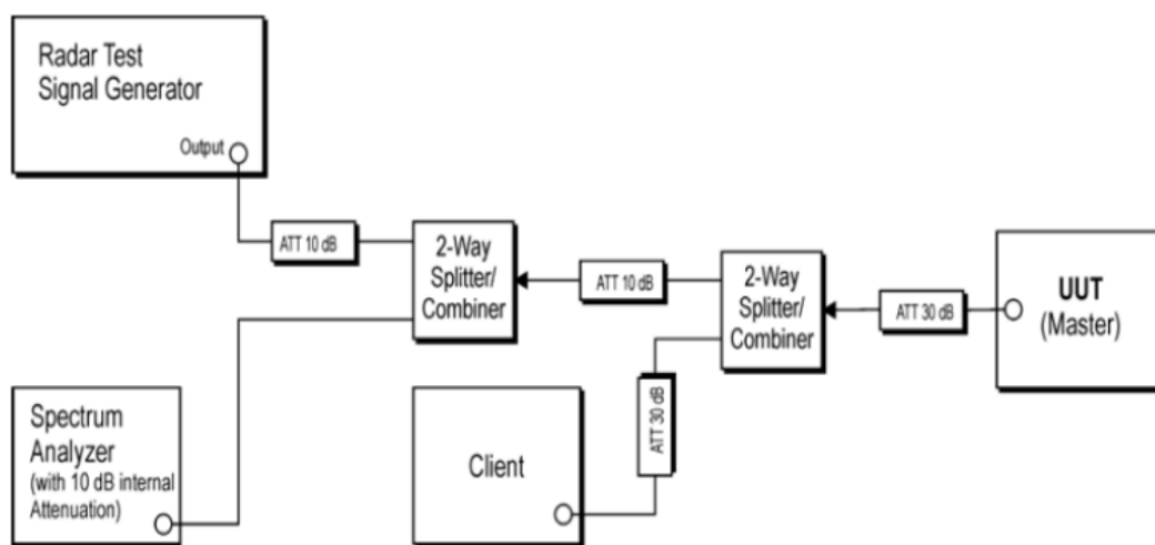
Figure 7-1. Test Setup
