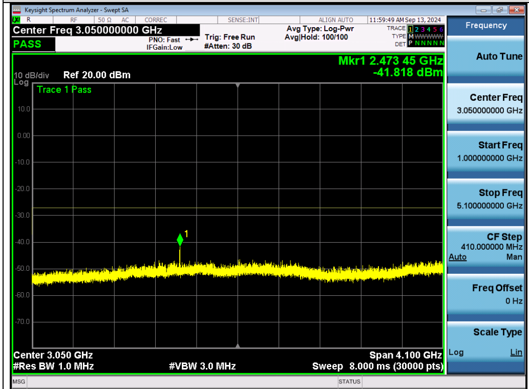
Test_Graph_802.11ac80_ANT1_5290_MCS0_Frequency Band 2
