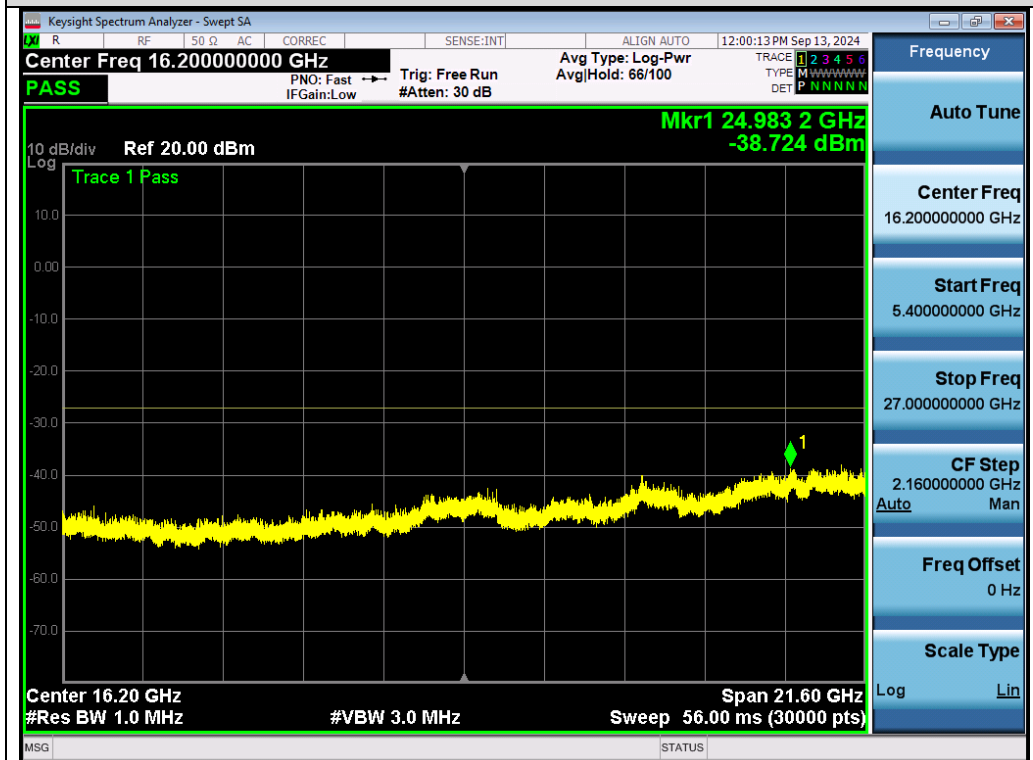
Test_Graph_802.11ac80_ANT1_5290_MCS0_Frequency Band 4
