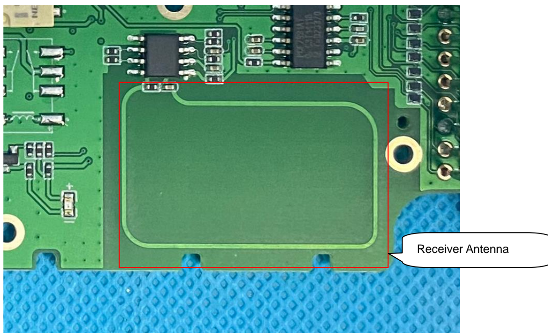
INTERNAL VIEW OF EUT (FIGURE 6)
