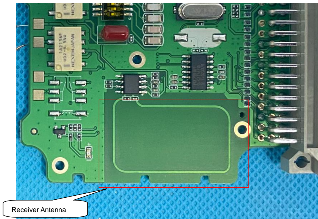
INTERNAL VIEW OF EUT (FIGURE 6)
