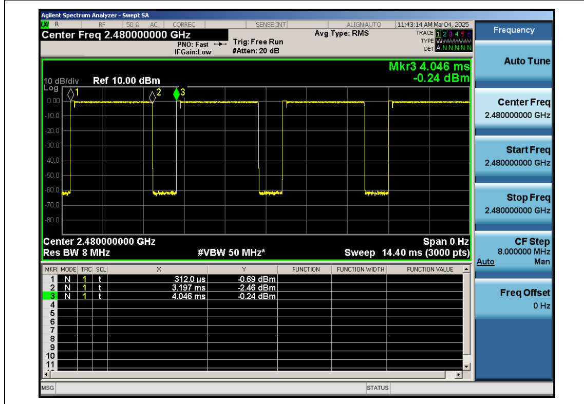
EDR-π /4-DQPSK-Ant1-2480
