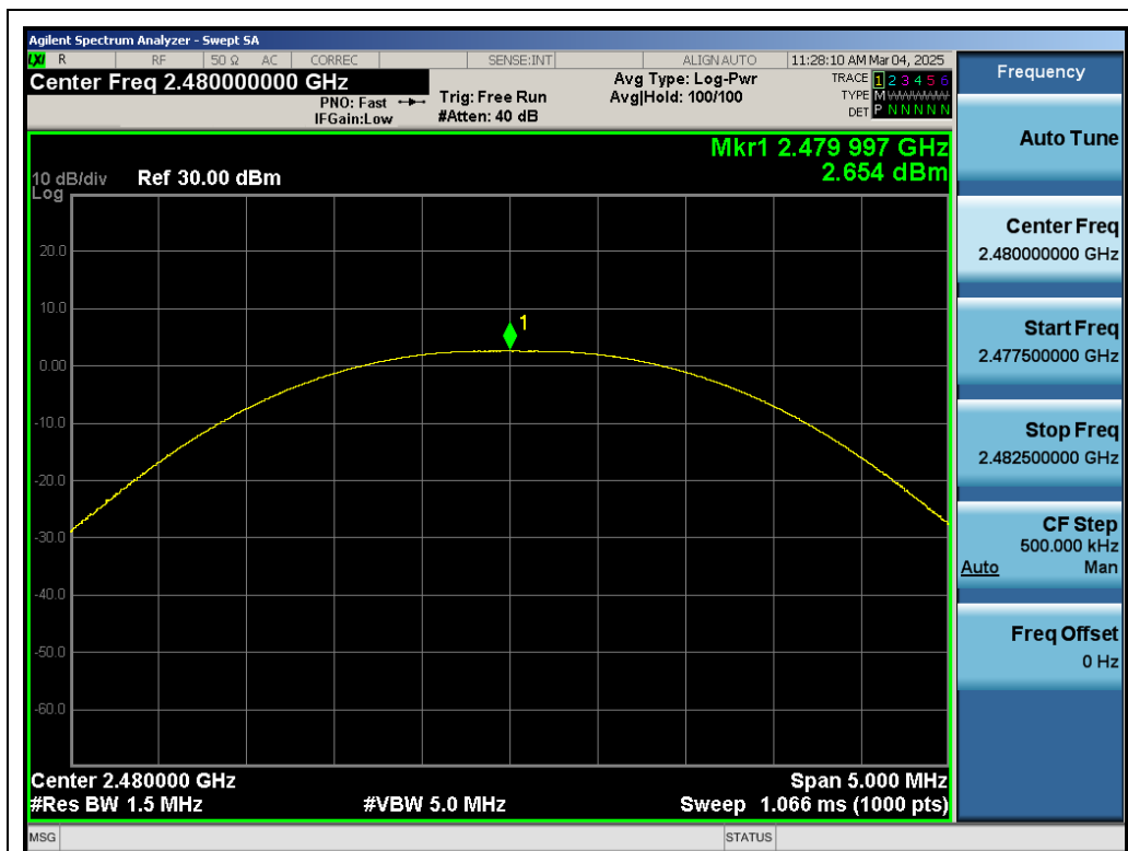
Test_Graph_BR_ANT1_2480_1Mbps_Peak Power
