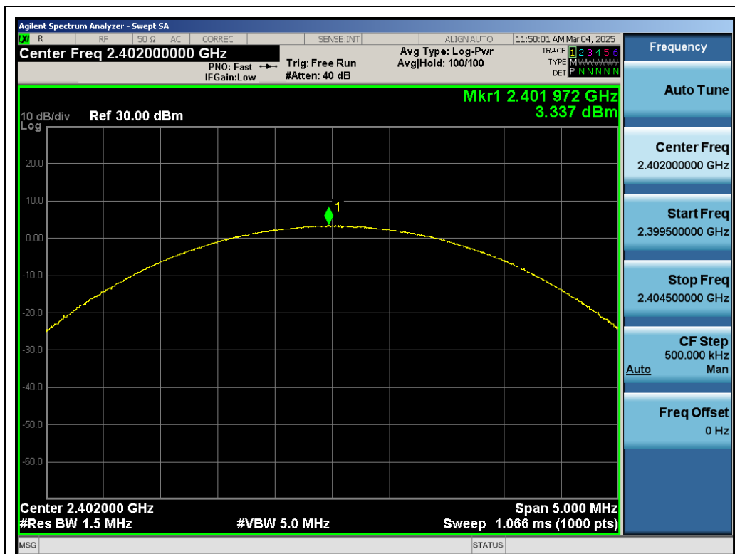
Test_Graph_EDR_ANT1_2402_3Mbps_Peak Power
