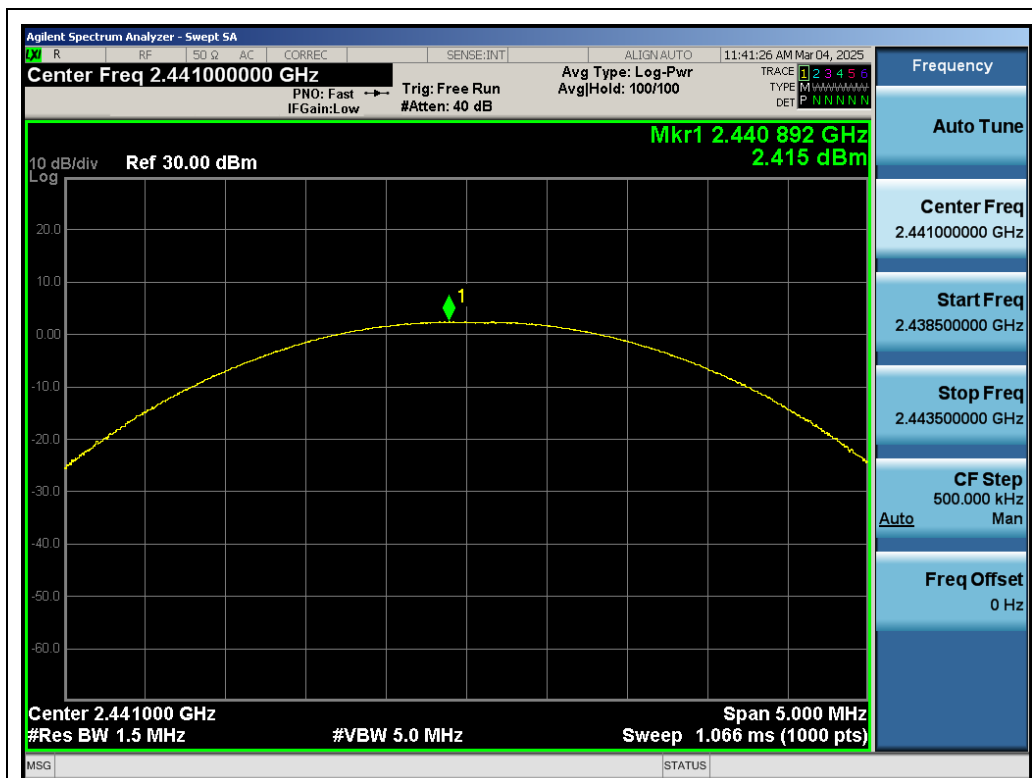
Test_Graph_EDR_ANT1_2441_2Mbps_Peak Power
