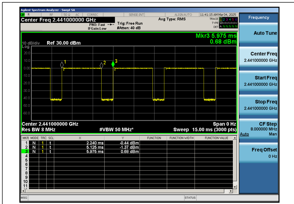
EDR-π /4-DQPSK-Ant1-2441
