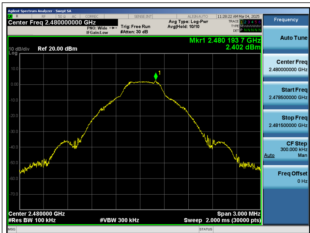
Test_Graph_BR_ANT1_2480_1Mbps_Reference Level
