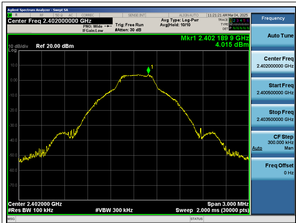
Test_Graph_BR_ANT1_2402_1Mbps_Reference Level
