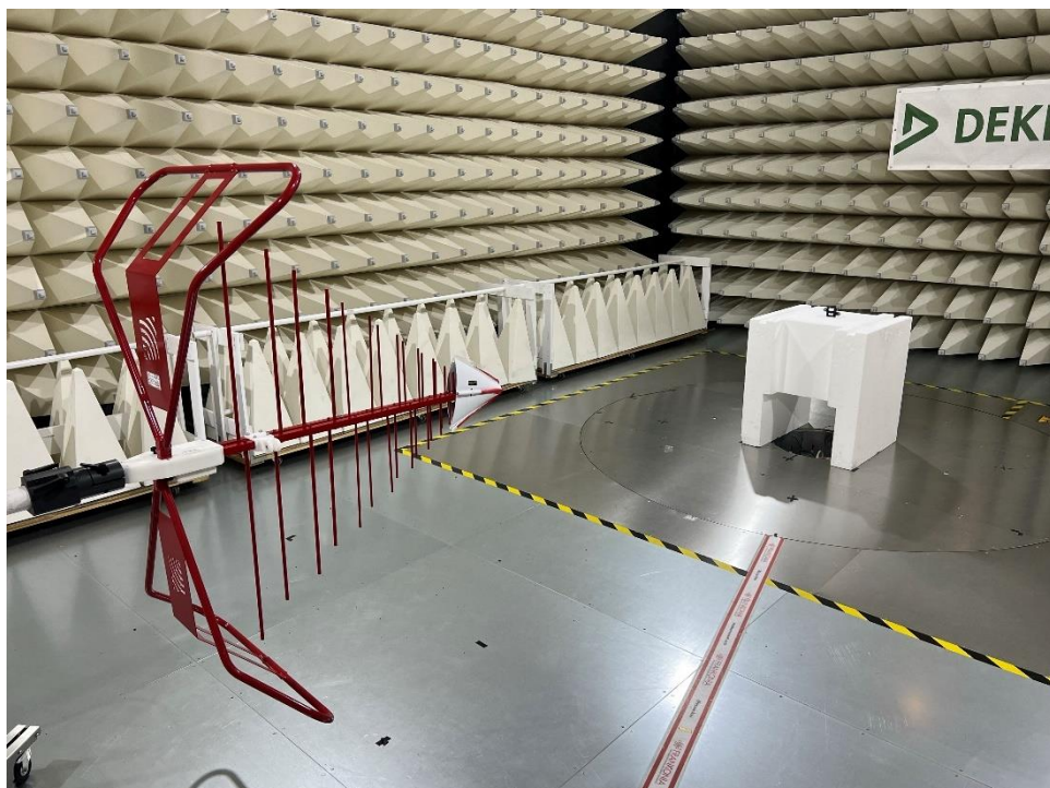
8. Low Range Radiated Emission test setup
