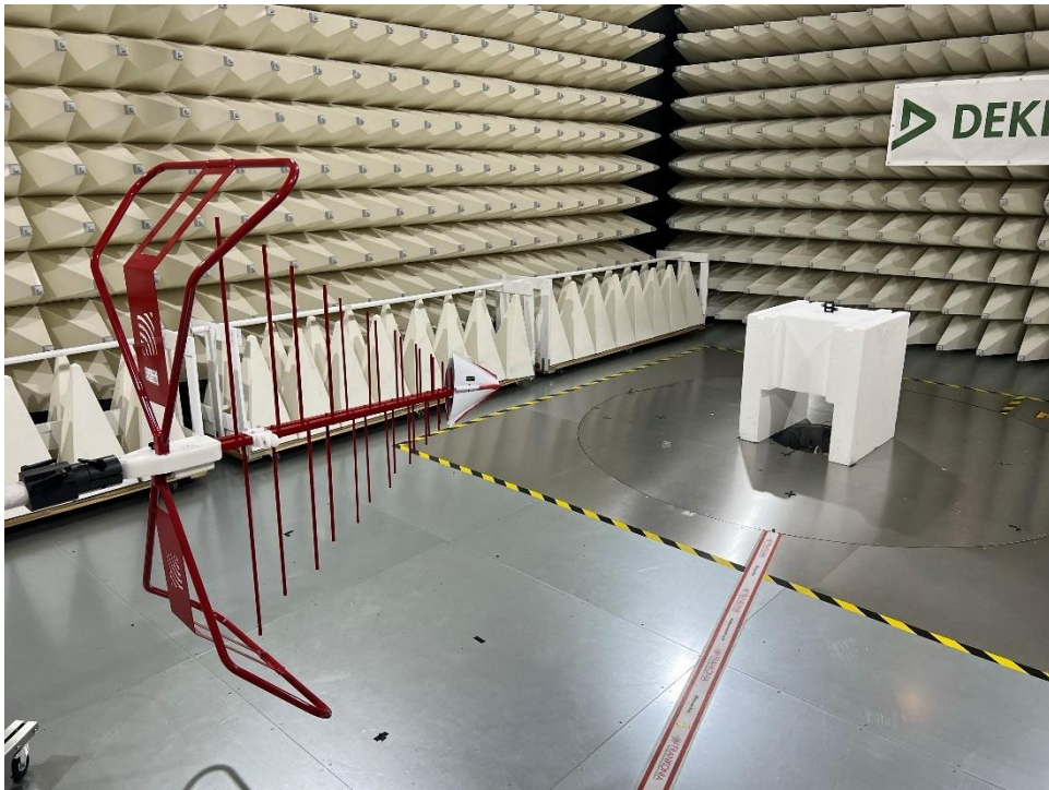
9. Low Range Radiated Emission test setup
