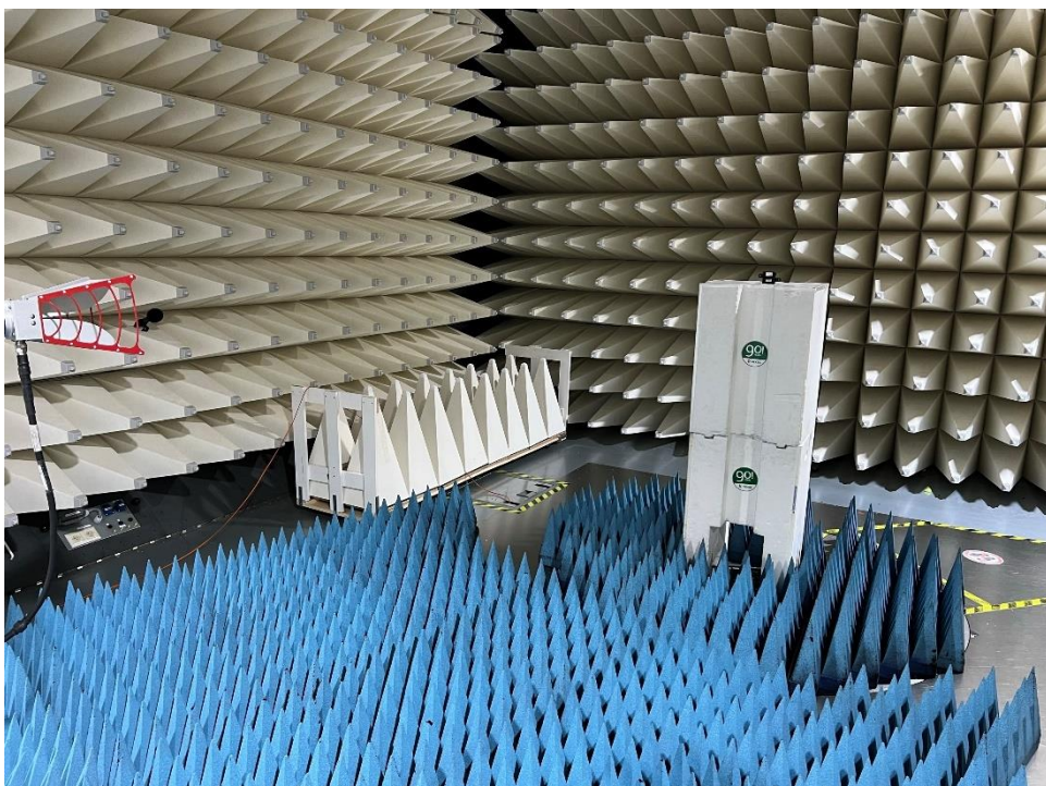
10. High Range Radiated Emission test setup
