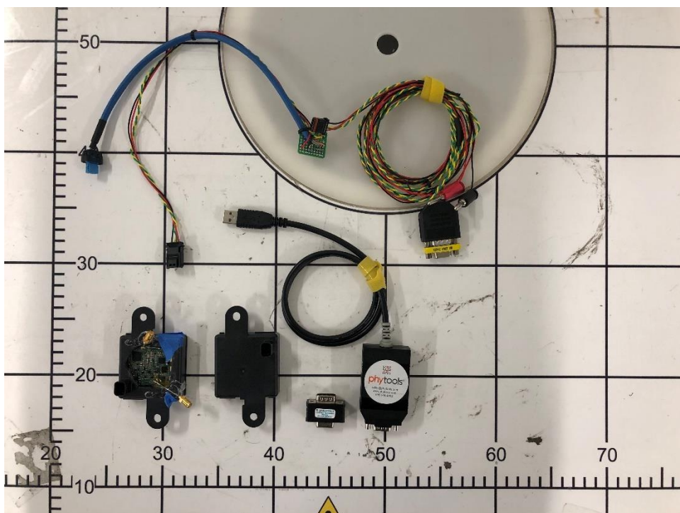
8. View of the Conducted and Radiated DUT with accessories
