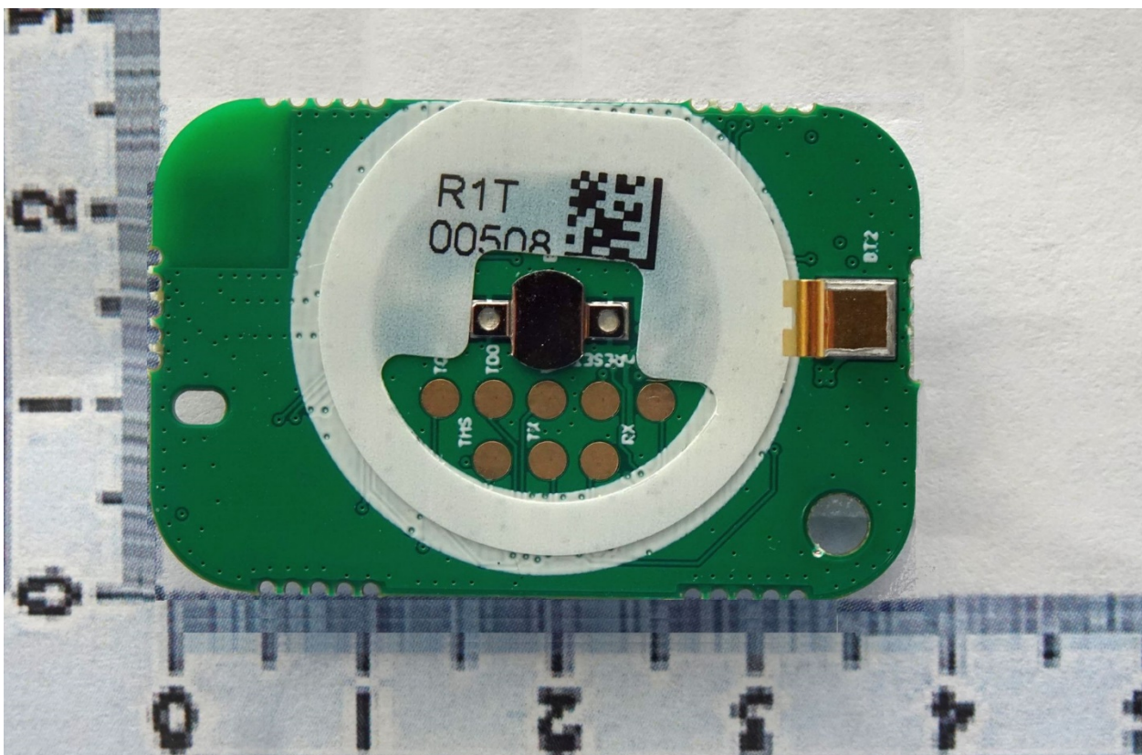
R1T KFB PCBA, Battery side View
