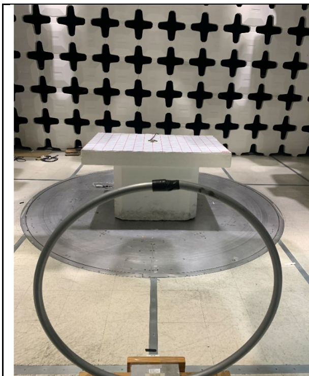
Radiated Emission Test below 30MHz Front View
