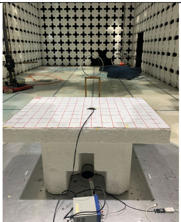
Radiated Emission Test below 30MHz Rear View
