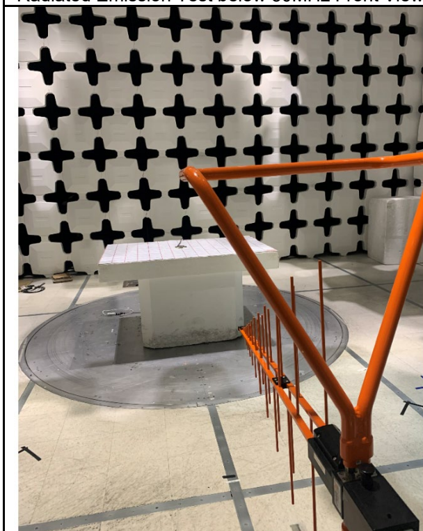
Radiated Emission Test below 1GHz Front View
