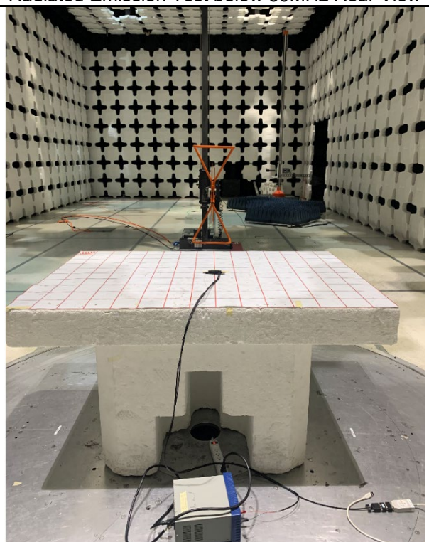
Radiated Emission Test below 1GHz Rear View
