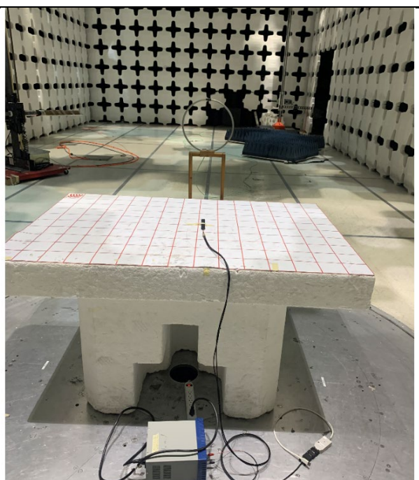
Radiated Emission Test below 30MHz Rear View
