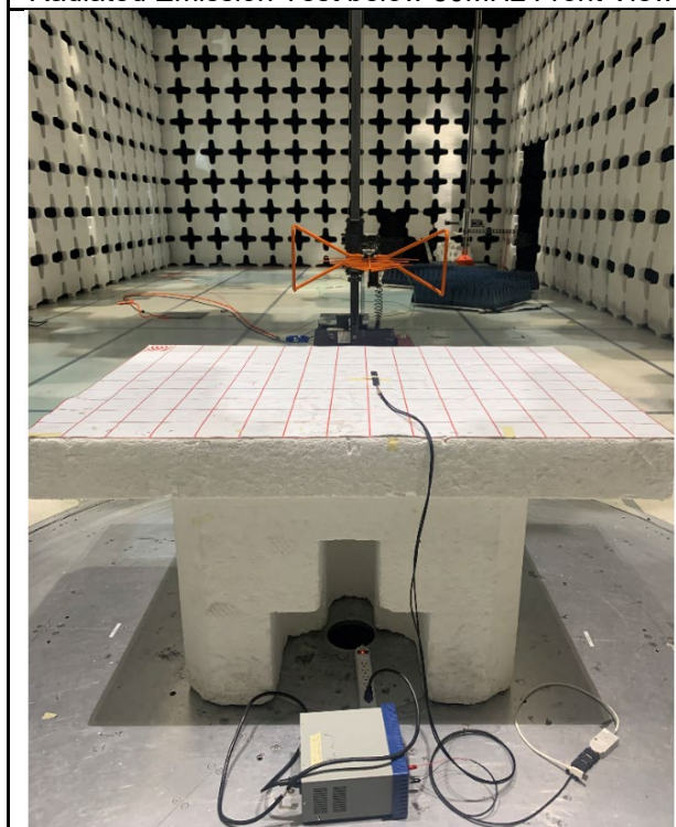
Radiated Emission Test below 1GHz Front View
