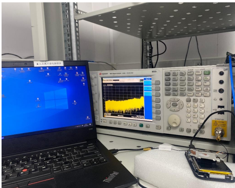
Conducted Test-2.4G WIFI
