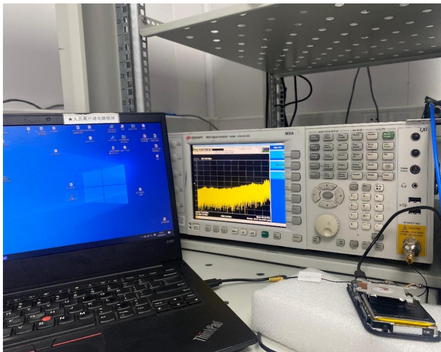
Conducted Test-BT
