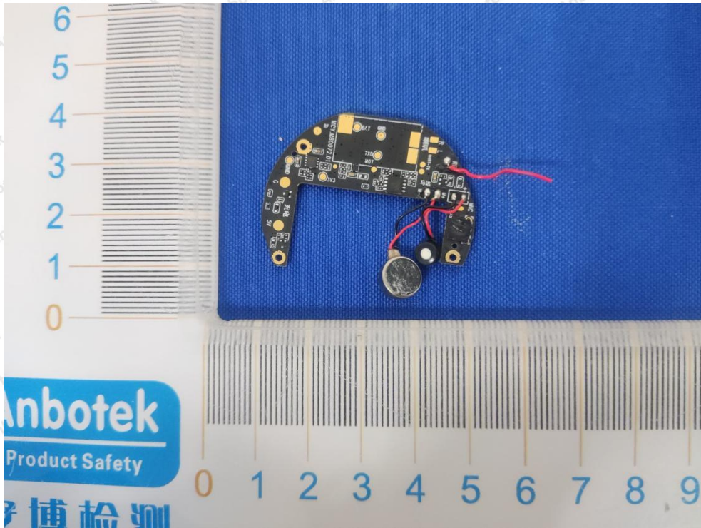
BDR+EDR ANT
