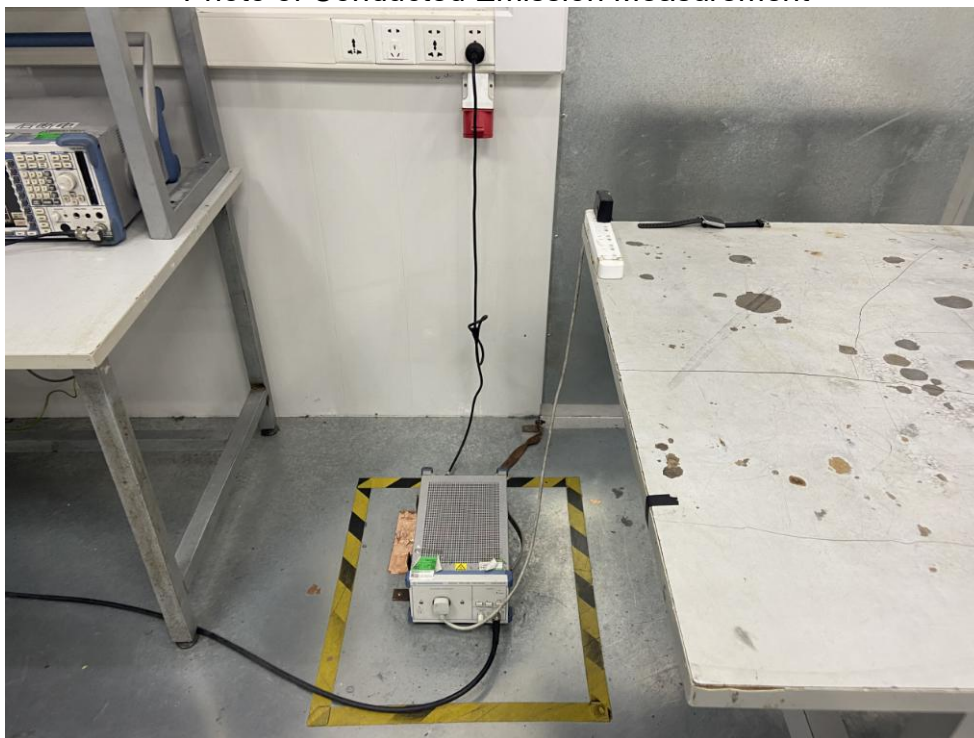
FCC ID: 2AW2F-ZW66 Photo of Conducted Emission Measurement
