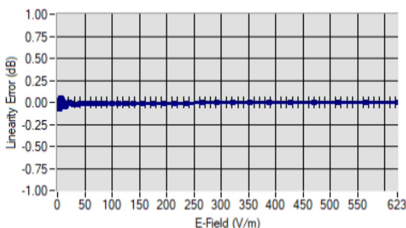
Linearity
