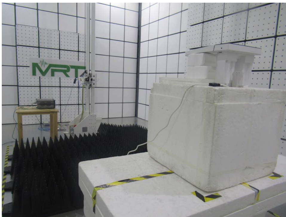
Photograph 4: Set-up photo for Radiated Spurious Emission, 18GHz ~ 40GHz
