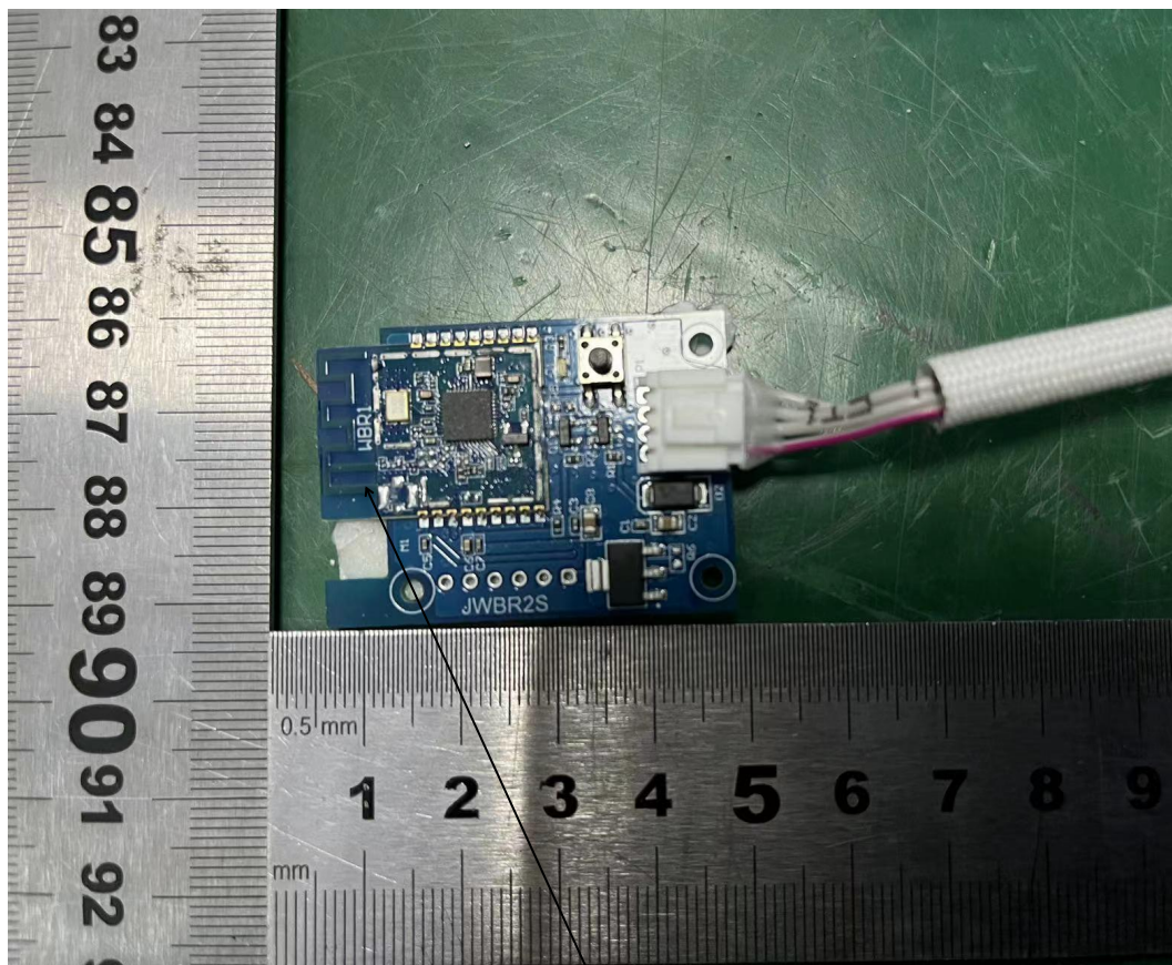
PCB ANTENNA
