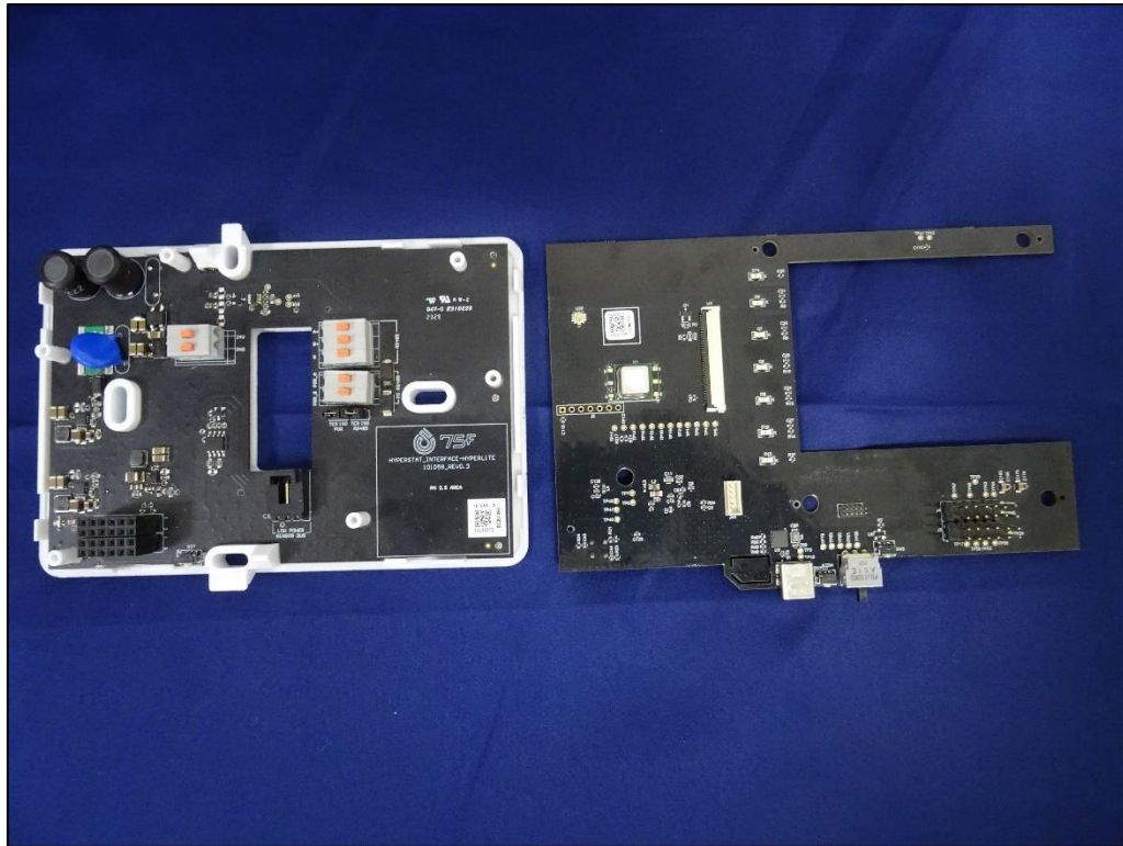
Picture 5 PCB Front and Rear View
