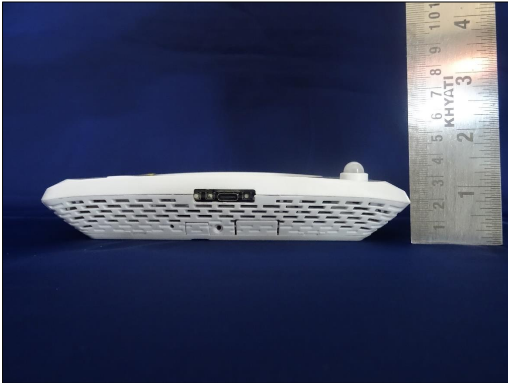
Picture 5 EUT Dimension View
