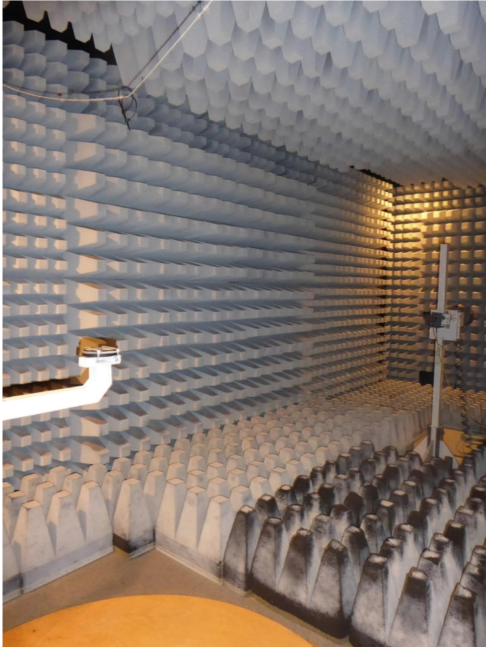
Test setup fully anechoic chamber TX spurious emissions from 12 GHz – 18GHz
