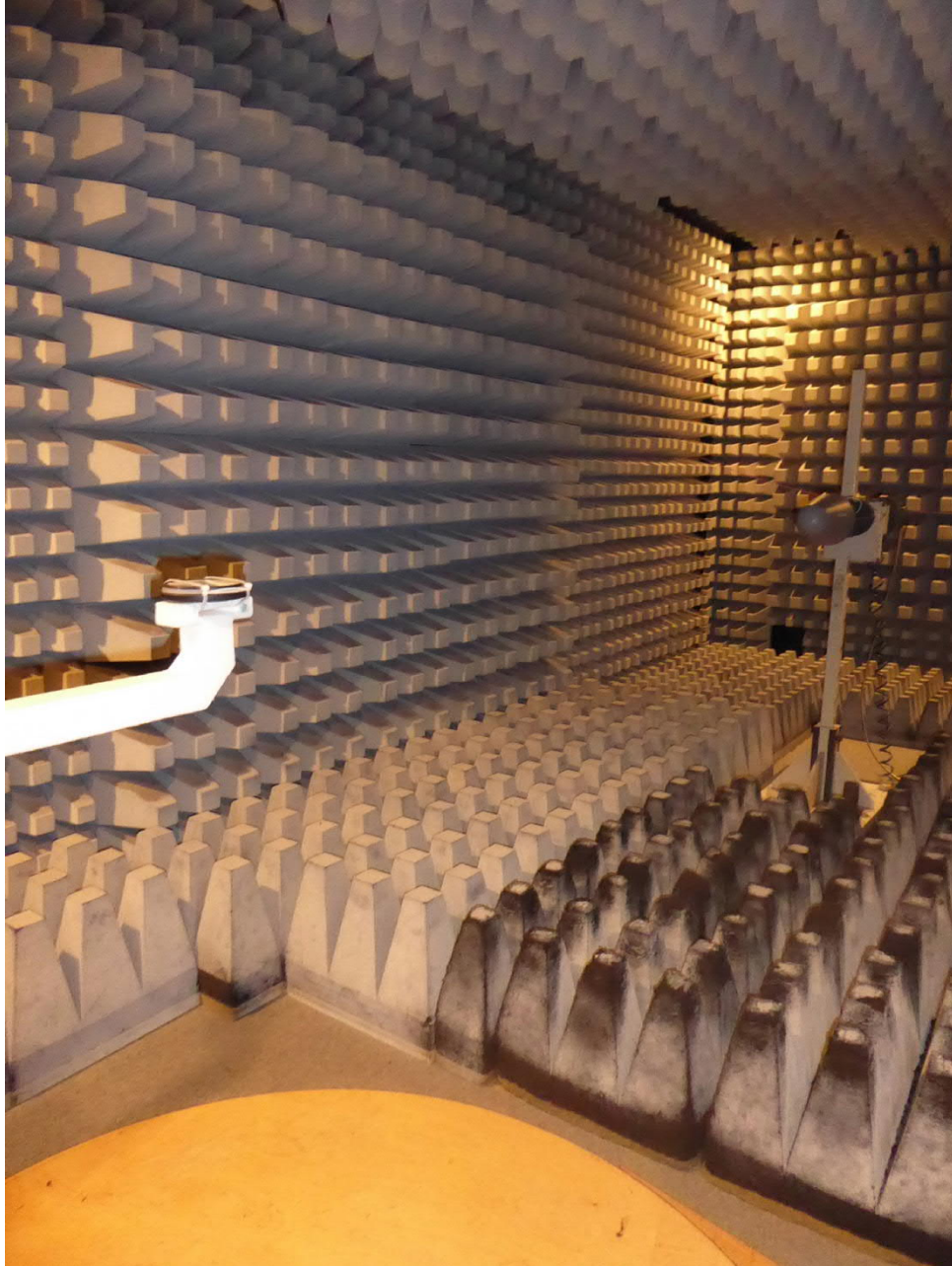
Test setup fully anechoic chamber TX spurious emissions from 1 GHz – 12GHz
