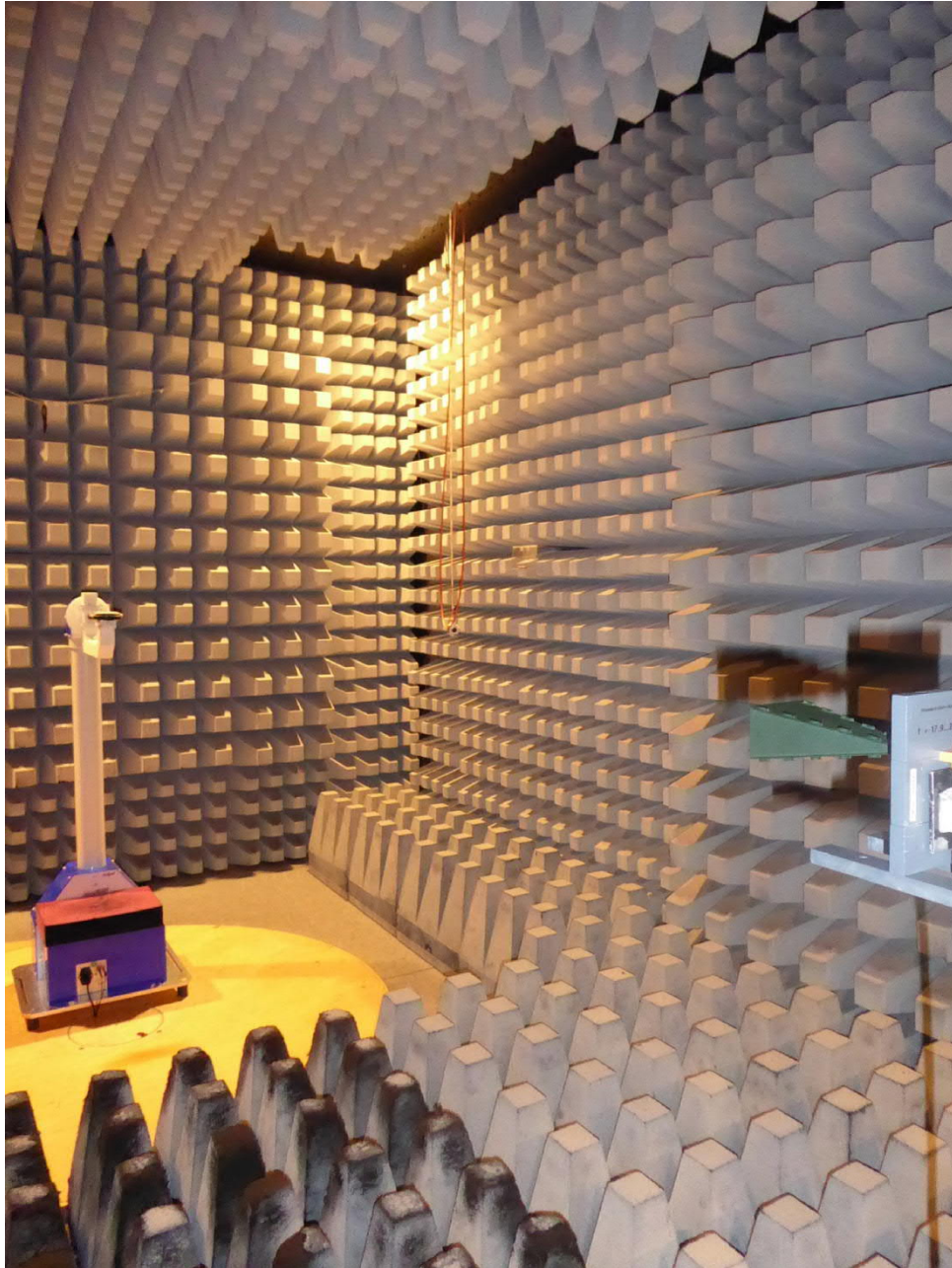
Test setup fully anechoic chamber TX spurious emissions from 18 GHz – 26.5 GHz
