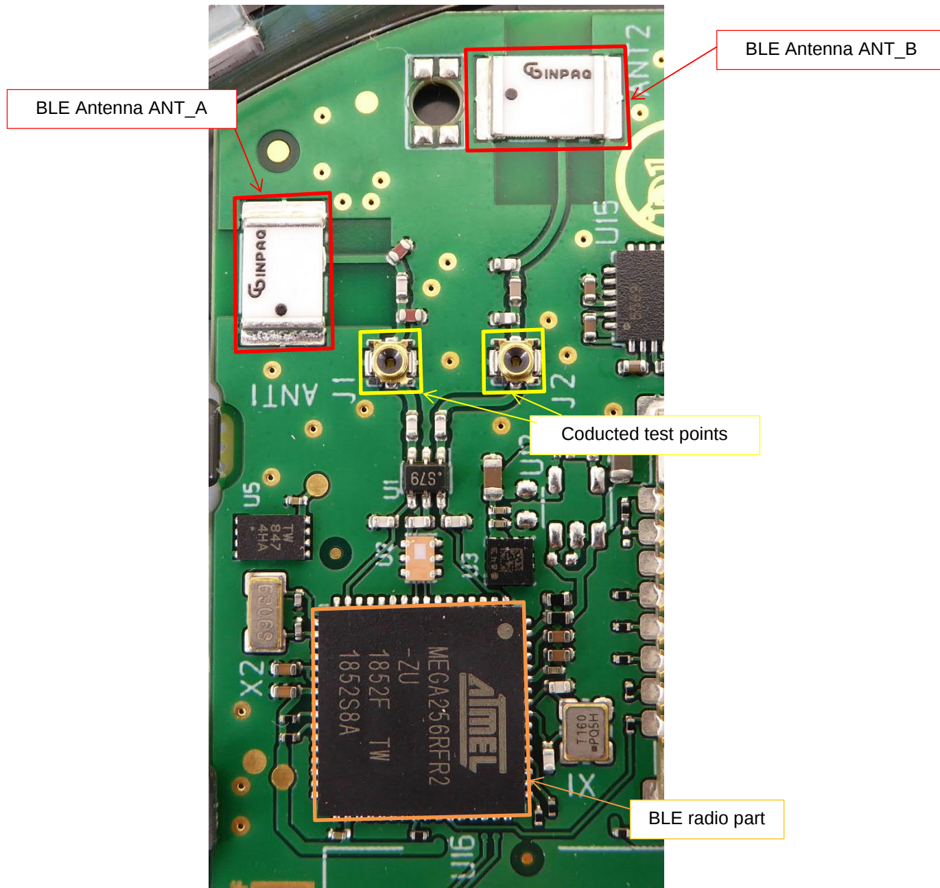
Radio Part IEEE802.15.4 (detail view)
