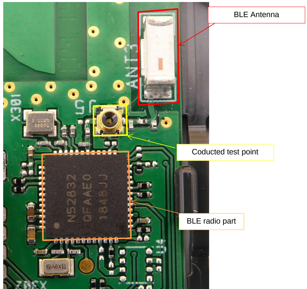
Radio Part BLE (detail view)
