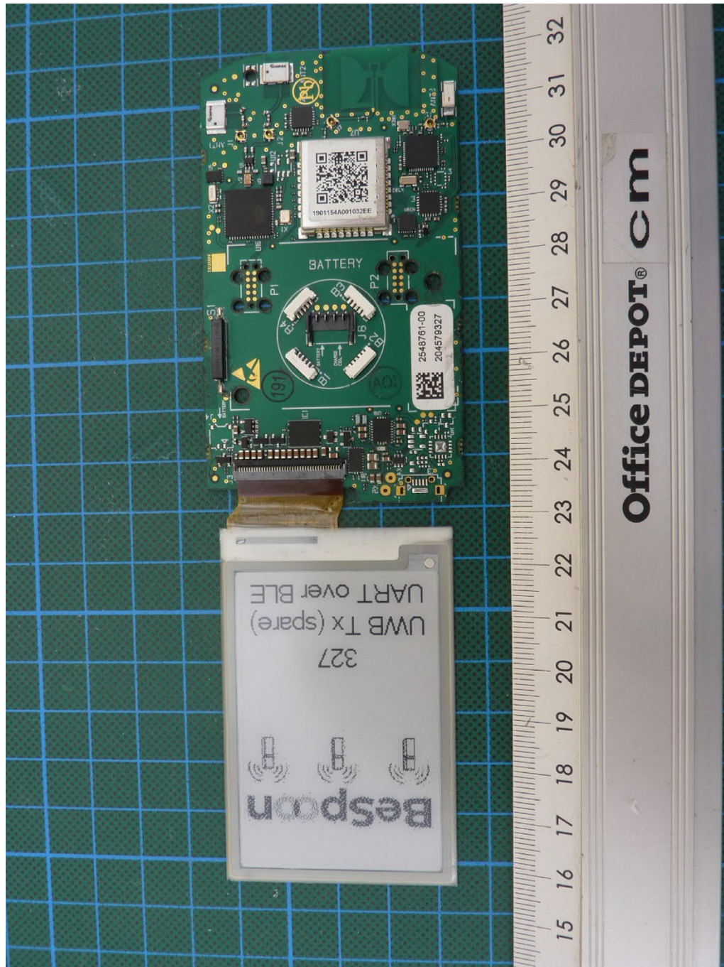
PCB with display, top view
