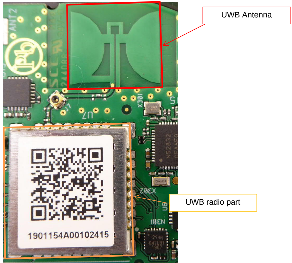
Radio Part UWB (detail view)
