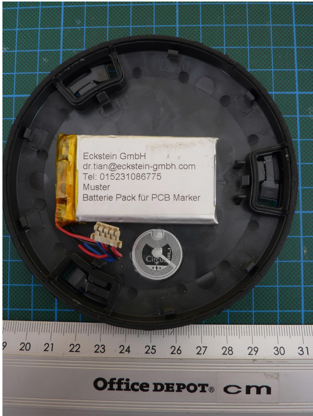
Housing, bottom part with battery
