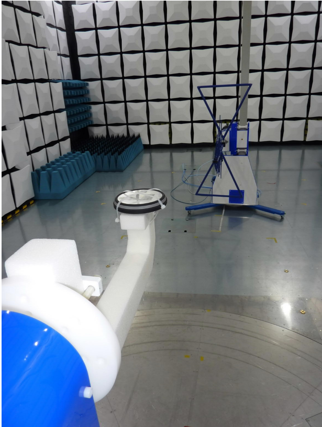
Test setup semi anechoic chamber TX spurious emissions from 30 MHz to 1 GHz
