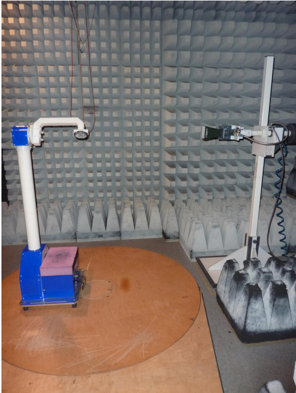
Test setup fully anechoic chamber TX spurious emissions from 1 GHz to 3.1 GHz and 10.6 to 40 GHz
