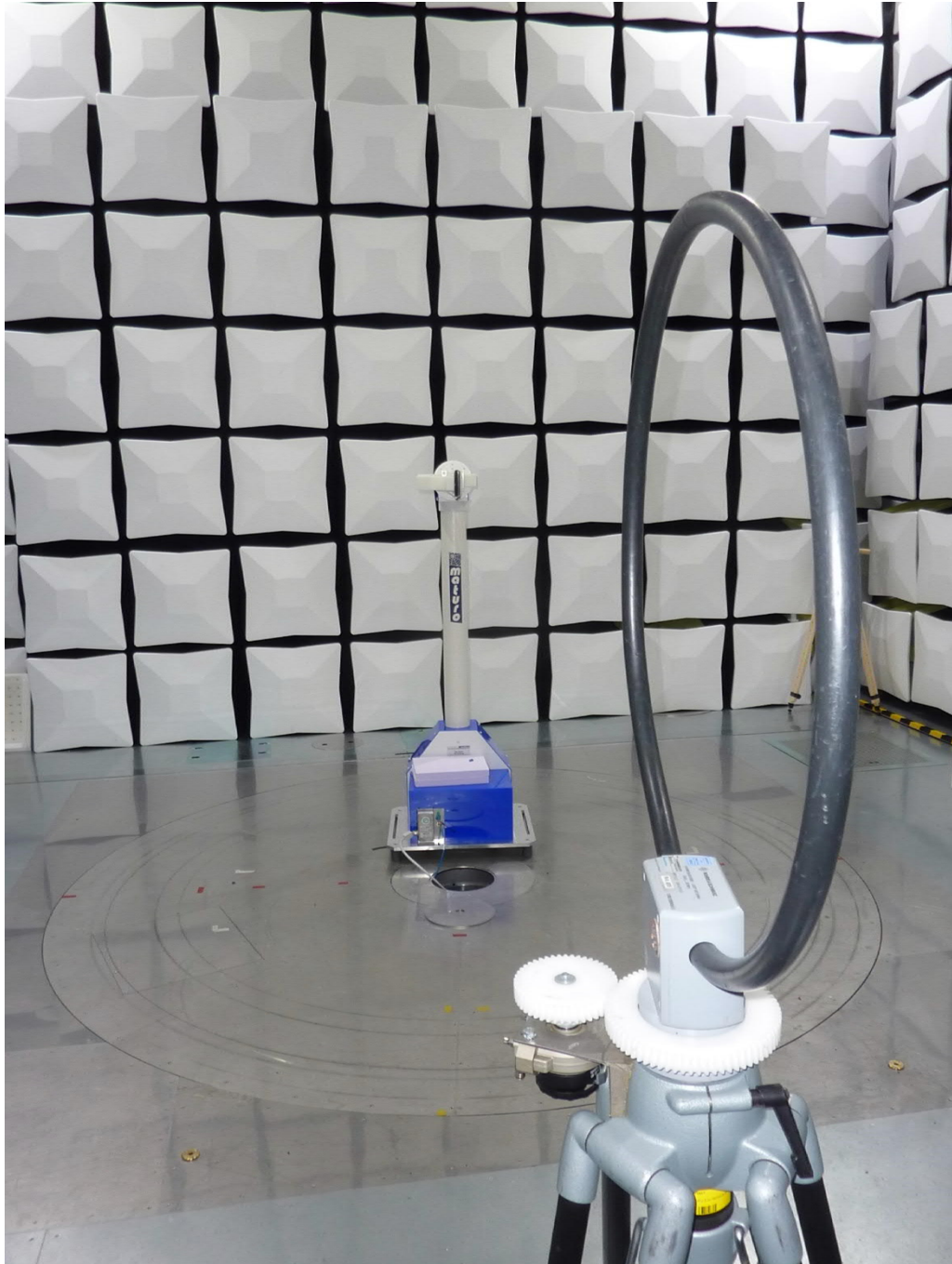
Test setup semi anechoic chamber TX spurious emissions from 10 MHz to 30 MHz
