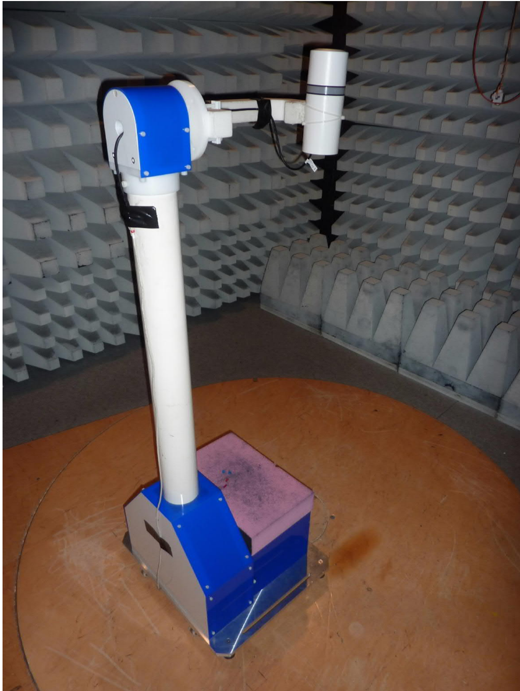
Test setup fully anechoic chamber TX spurious emissions from 1 GHz to 40 GHz
