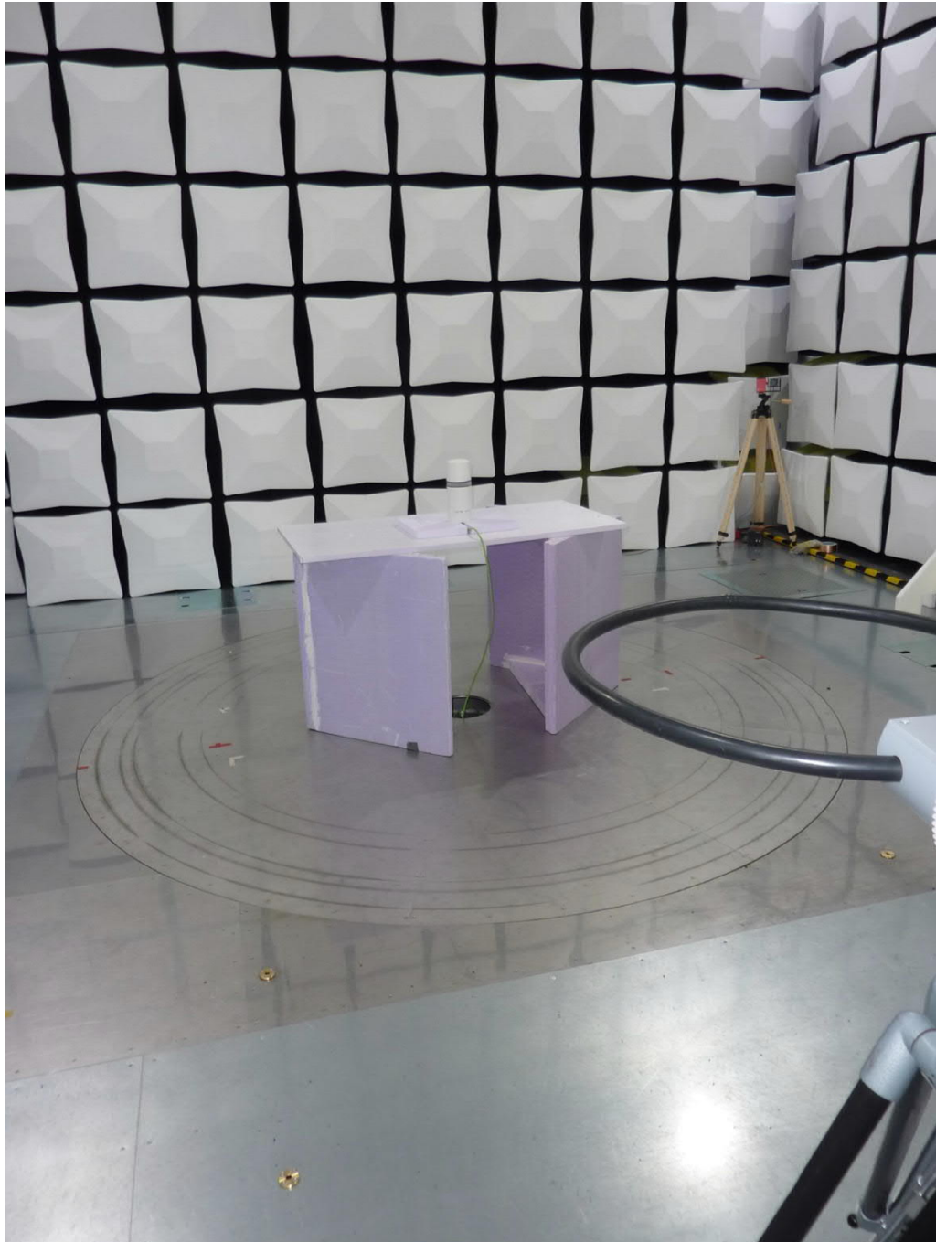
Test setup semi anechoic chamber TX spurious emissions from 9 kHz to 30 MHz
