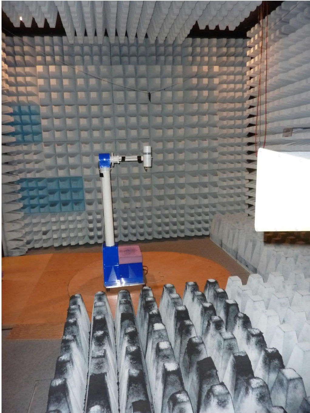
Test setup fully anechoic chamber TX spurious emissions from 3.1 GHz to 10.6 GHz
