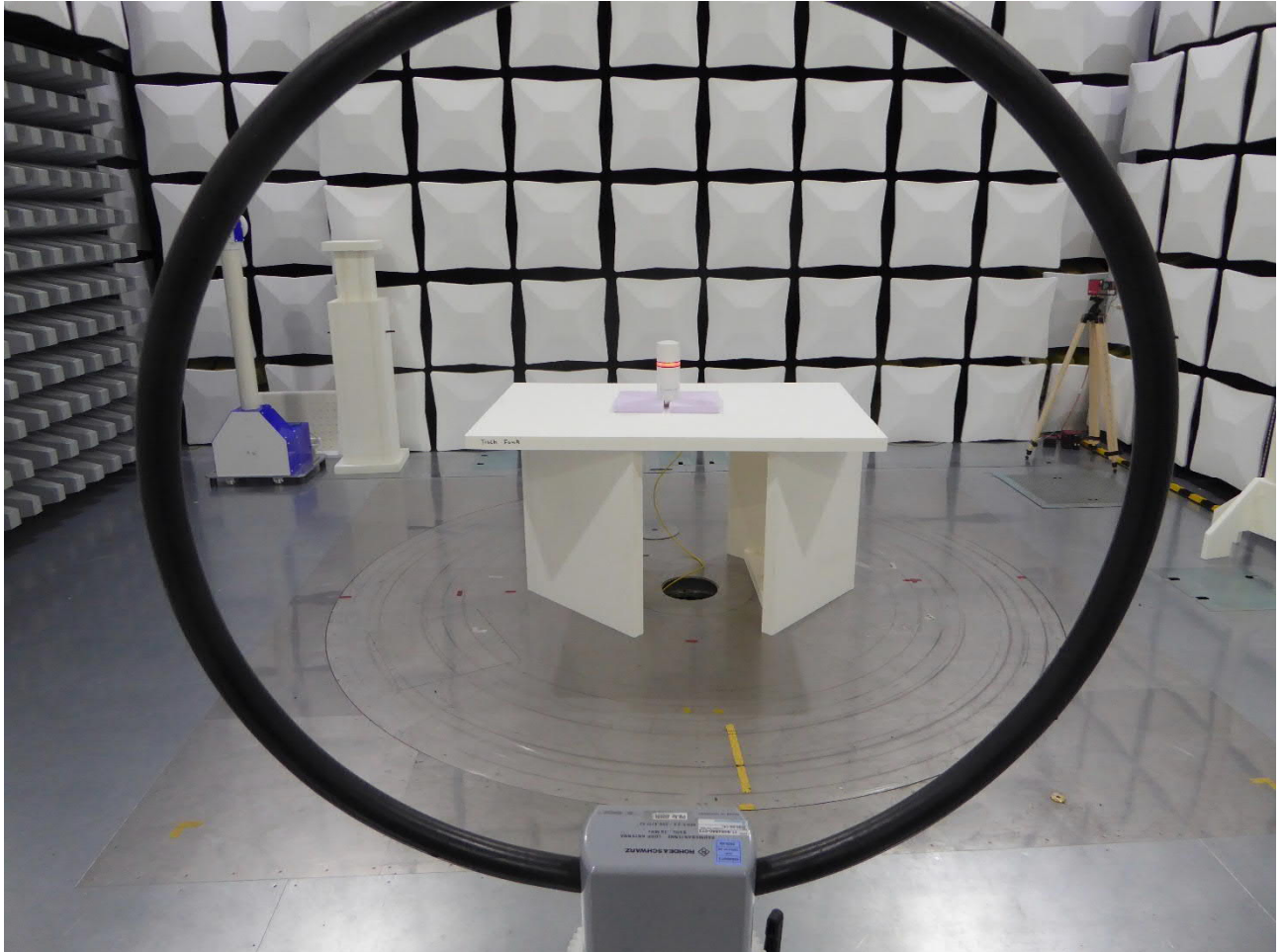
Test setup semi anechoic chamber TX spurious emissions from 9 kHz to 30 MHz
