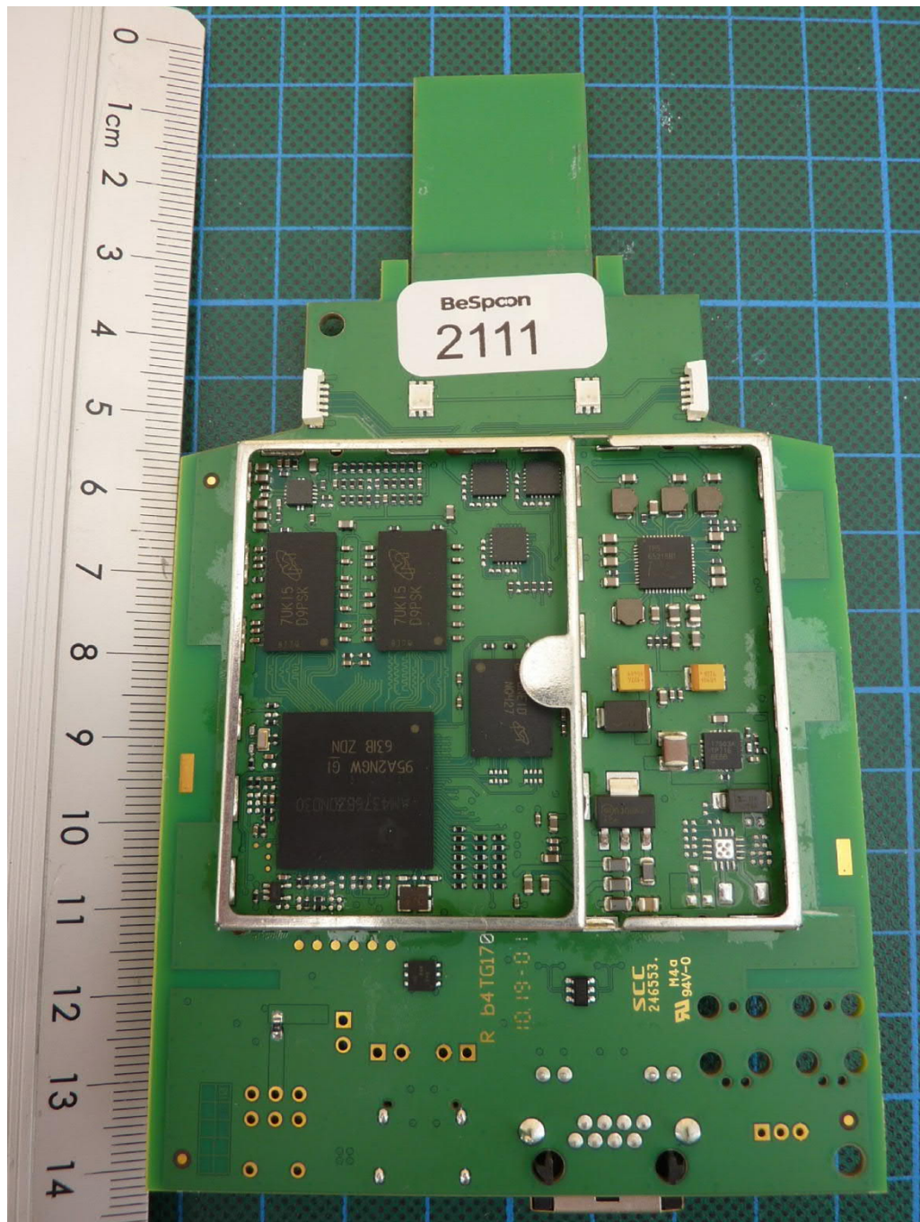
PCB, bottom view (shielding removed)
