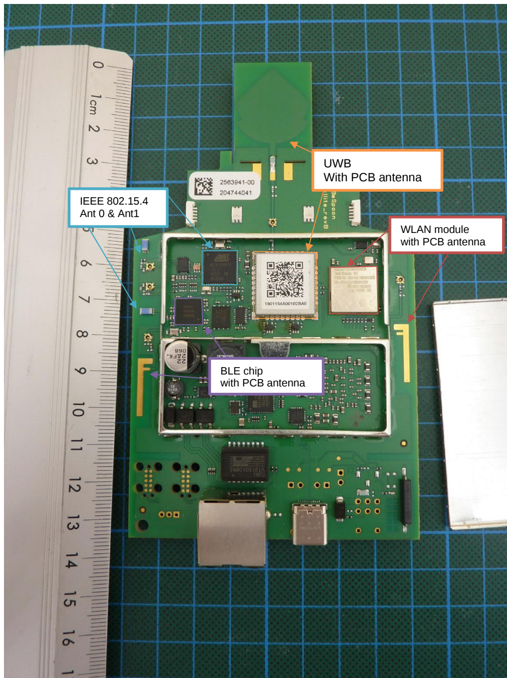
PCB, top view (shielding removed) With module information
