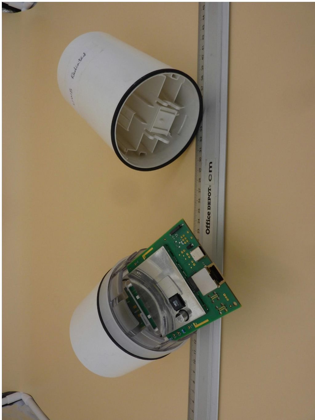
Internal view 1 (housing opened)
