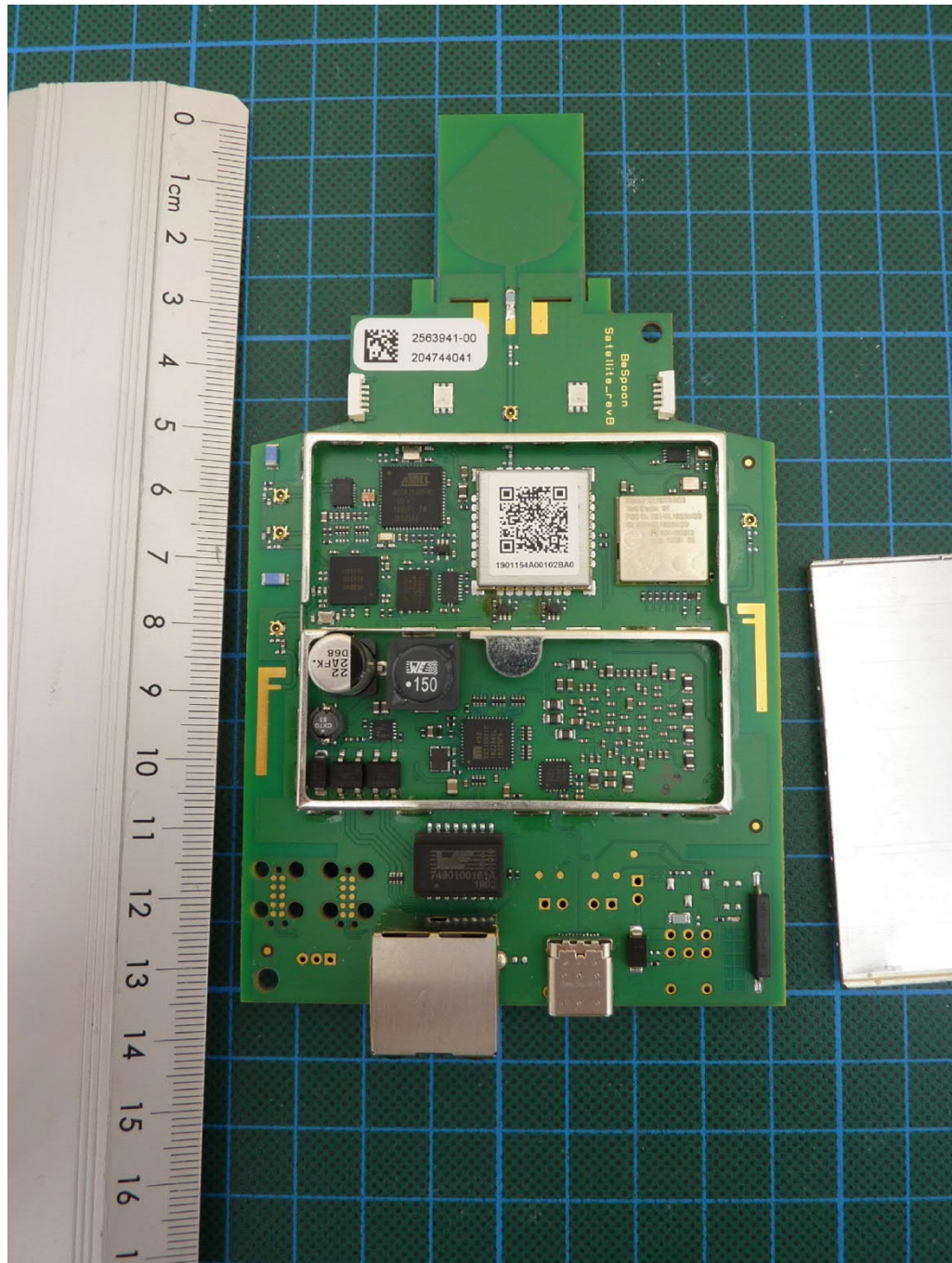
PCB, top view (shielding removed)
