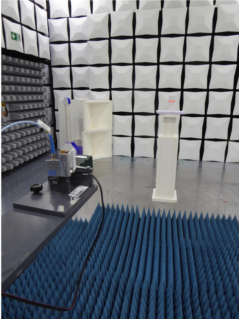
Test setup semi anechoic chamber TX spurious emissions from 18 GHz – 26.5 GHz
