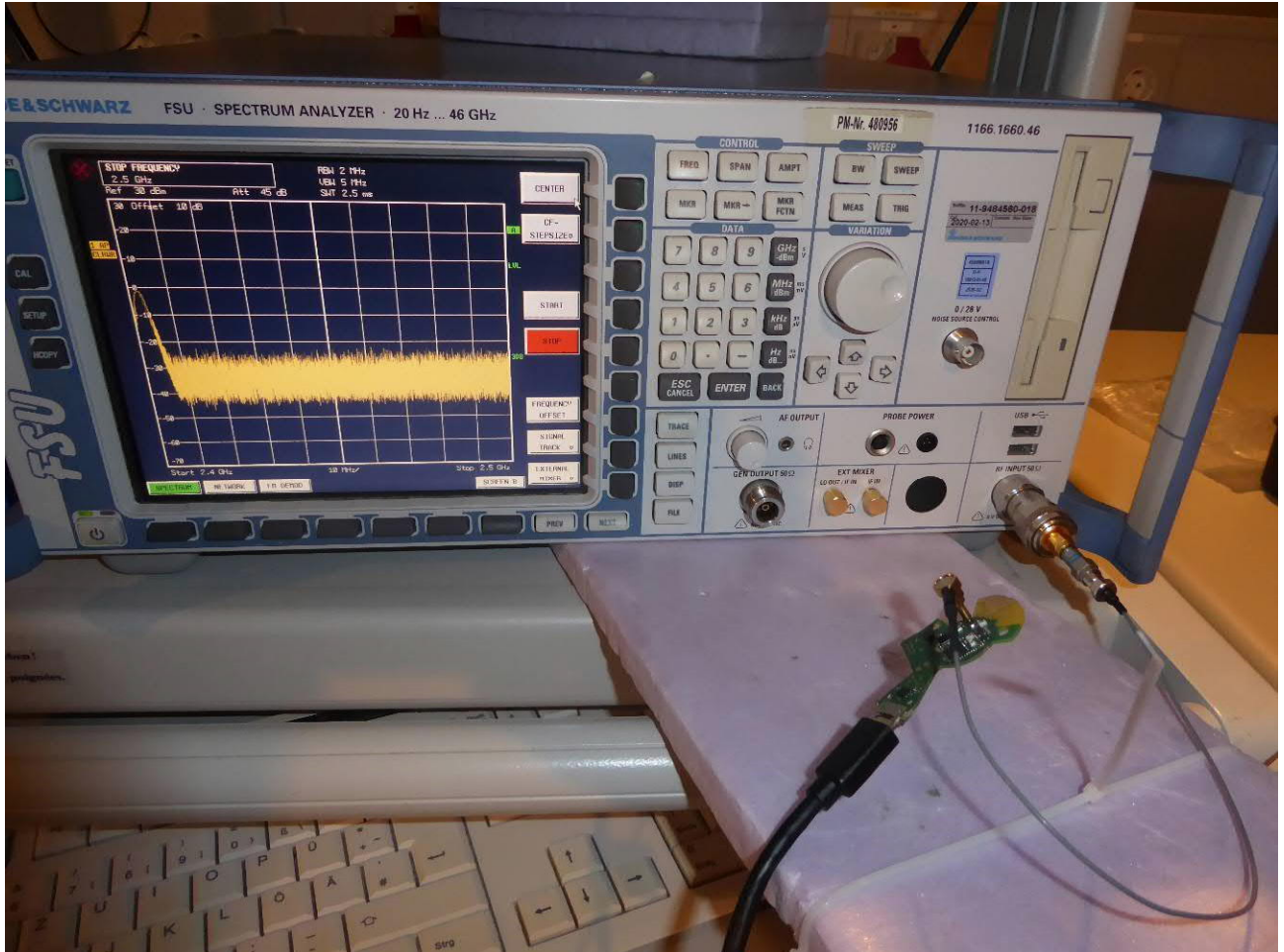
Test setup SmartAntenna – antenna port conducted test in shielded chamber
