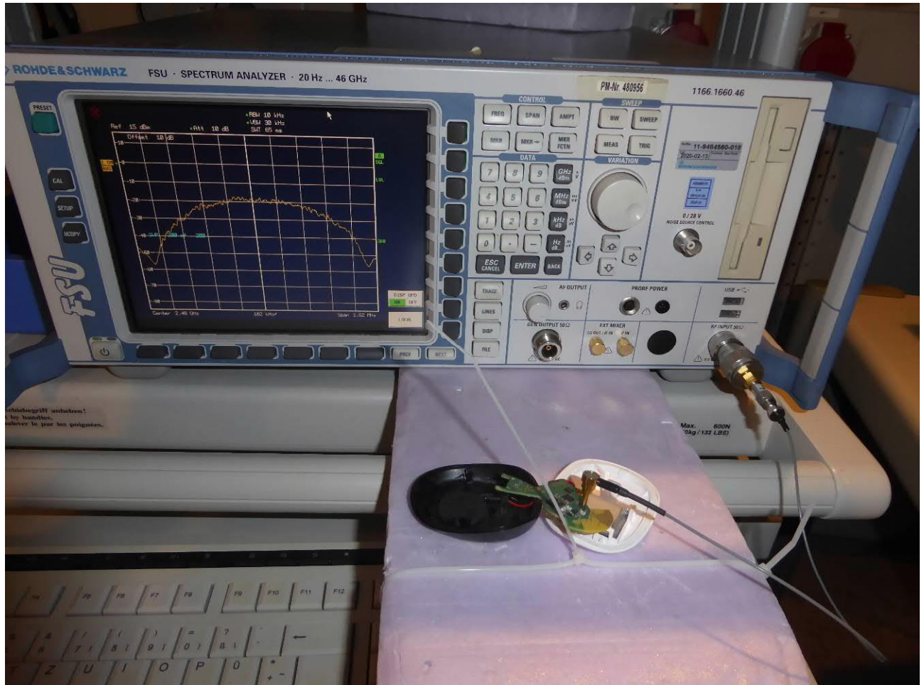
Test setup WTag – antenna port conducted test in shielded chamber
