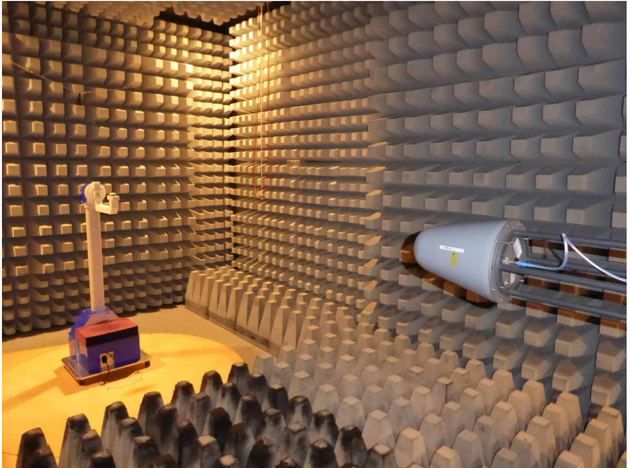
Test setup WTag – radiated test in anechoic chamber (M20)
