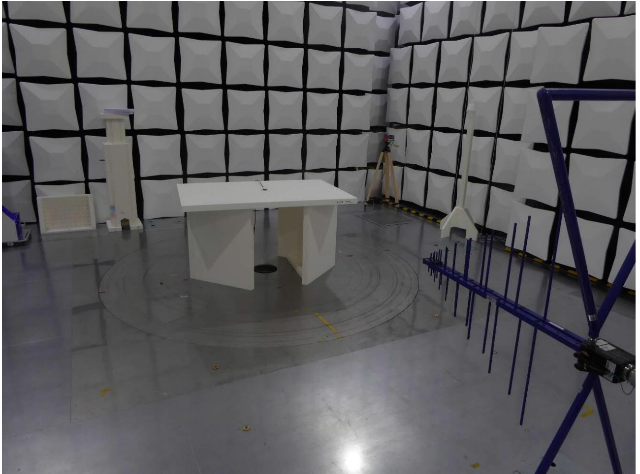
Test setup SmartAntenna – radiated test in anechoic chamber (M276)
