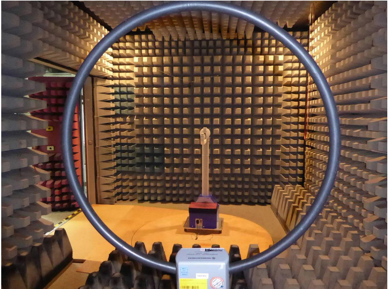
Test setup SmartAntenna – radiated test in anechoic chamber (M20)
