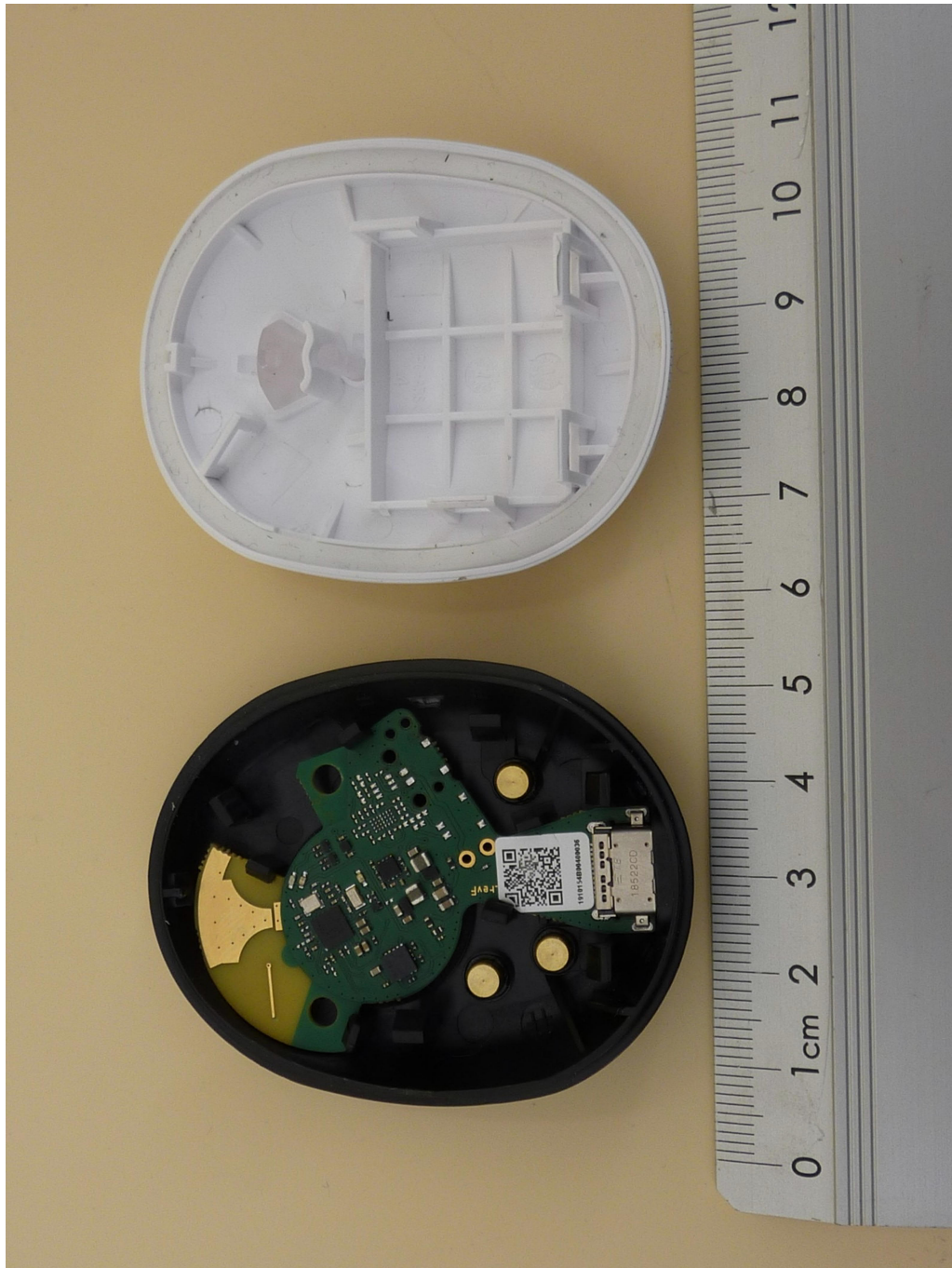
omlox SmartAntenna, internal view 1
