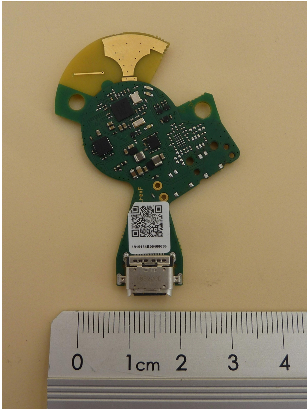
omlox SmartAntenna, PCB, top view
