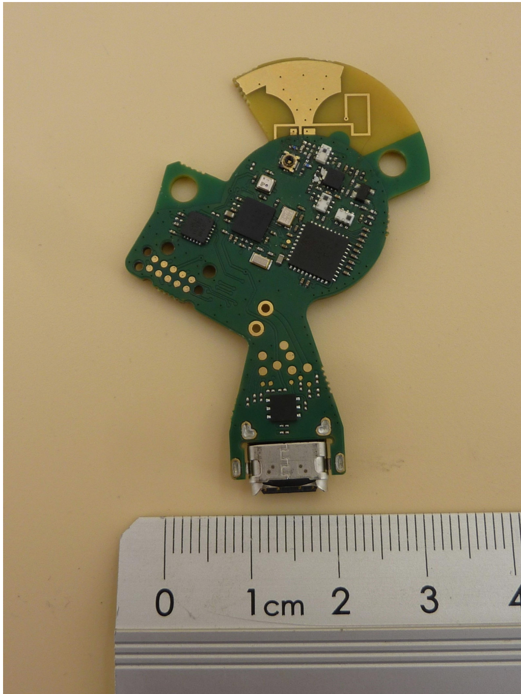
omlox SmartAntenna, PCB, bottom view
