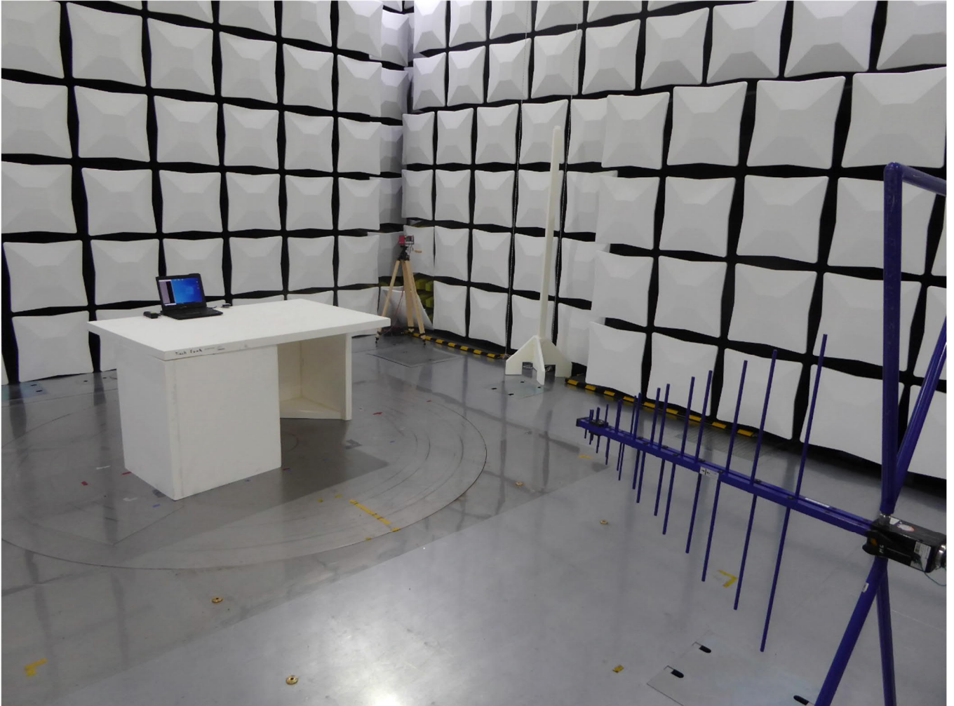
Test setup SAC radiated emission 30 MHz -1000 MHz
