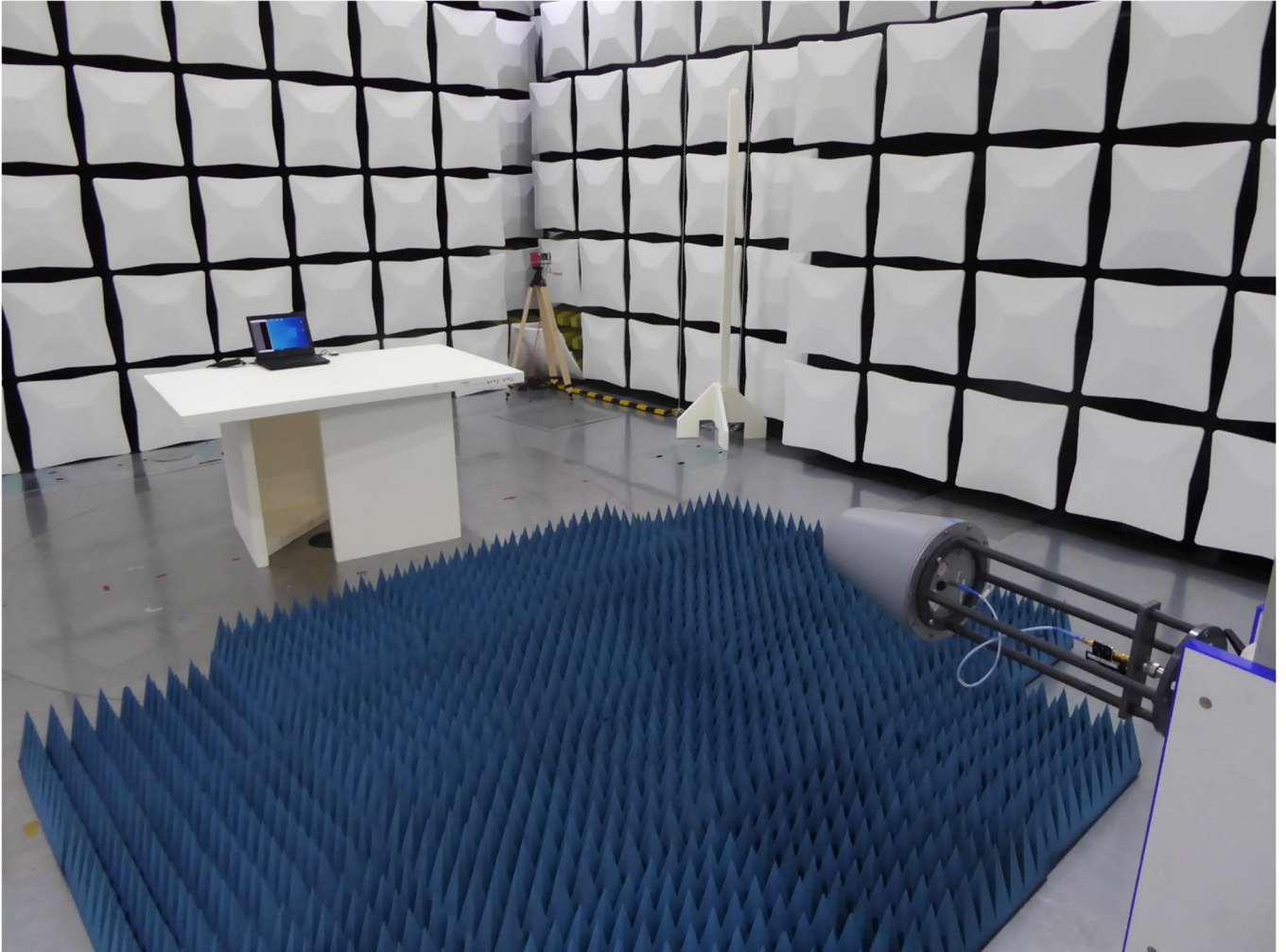
Test setup SAC with floor absorbers radiated emission 1 GHz - 12 GHz
