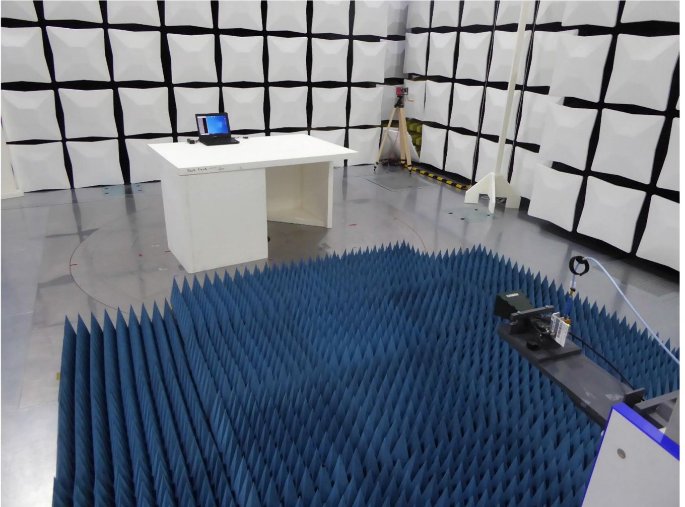
Test setup SAC with floor absorbers radiated emission 12 - 18 GHz
